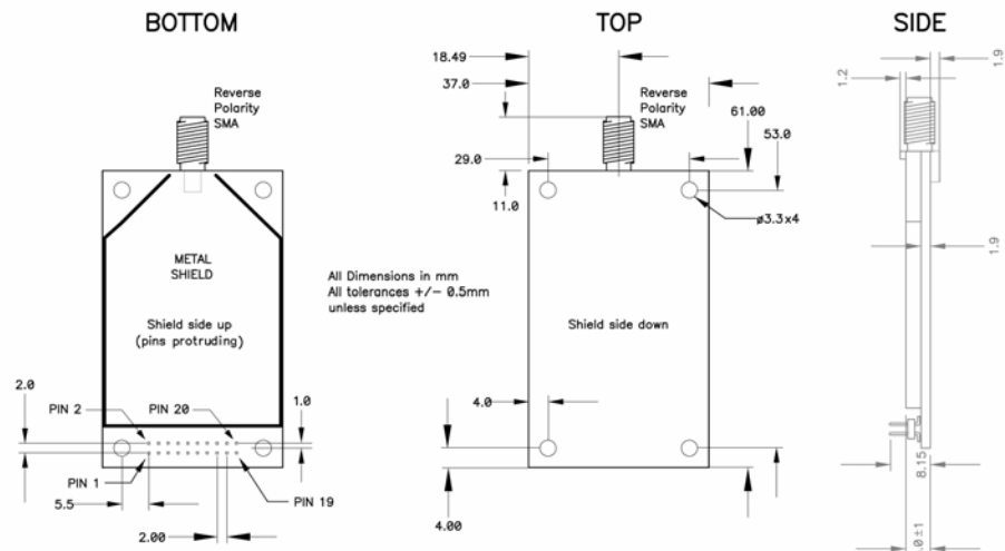
Figure 1.5. XTend Module Mechanical Drawings (with RPSMA antenna connector)
