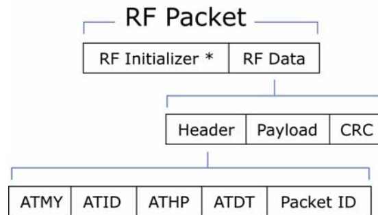
Figure 2.5. RF Packet Components
