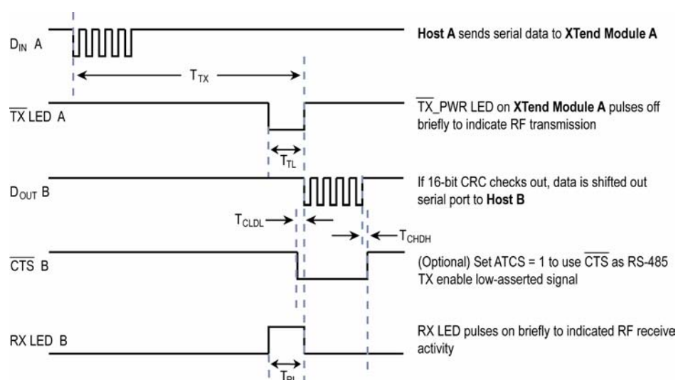
Figure 1.3. Timing Specifications (“A” and “B” refer to Figure 1.2)
