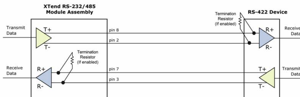
Figure B.21. XTend Module Assembly in an RS-485 (4-wire) environment
