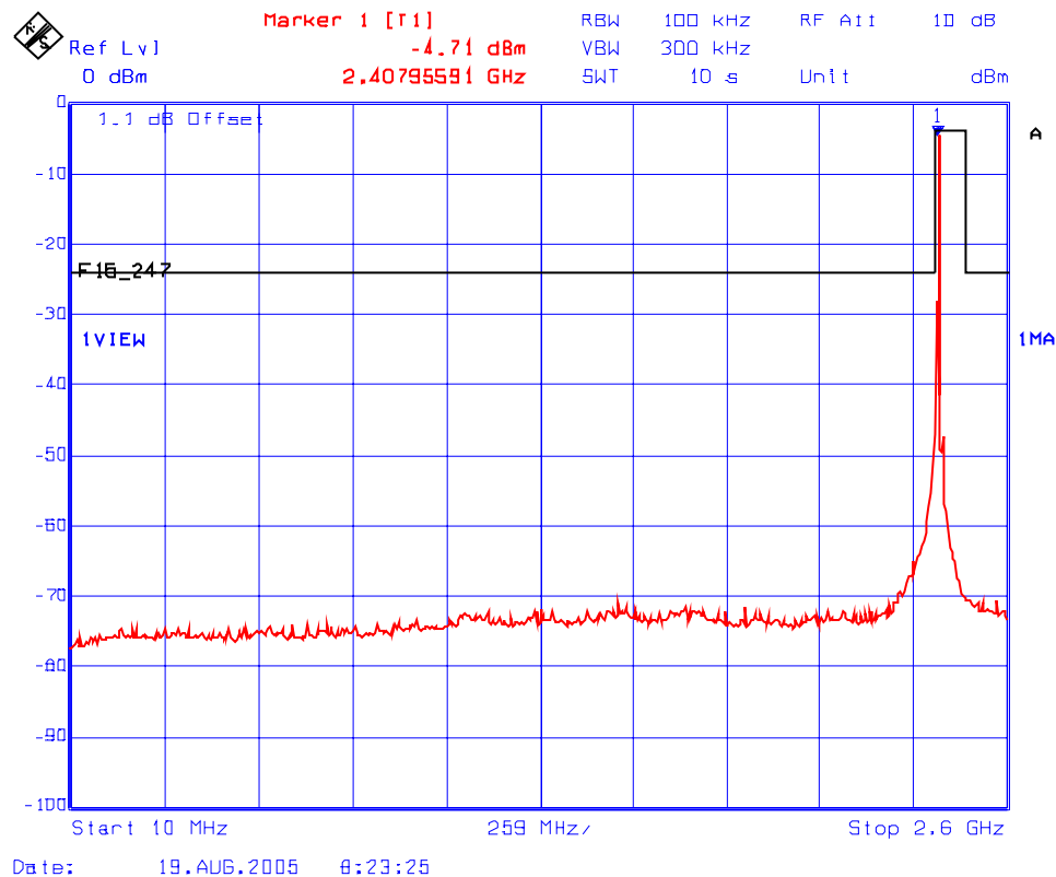
Plot#10: Spurious RF Conducted Emissions Transmitter Frequency: 2405 MHz
