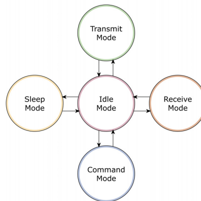
Figure 2-04. XBee/XBee-PRO RF Module Modes of Operation (The RF Modules operate in one mode at a time.)
