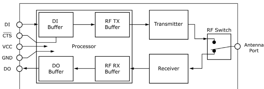
Figure 2-03. Internal Data Flow Diagram
