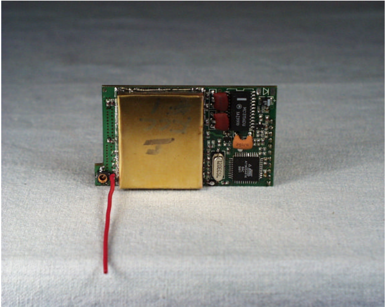
Small Dipole Antenna
