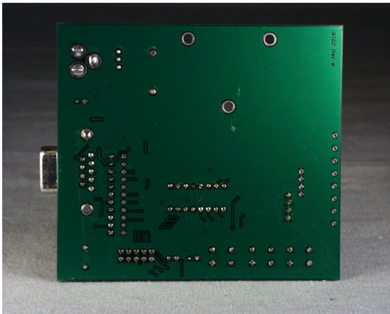
Back View of the 9XTREAM and Interface Board
