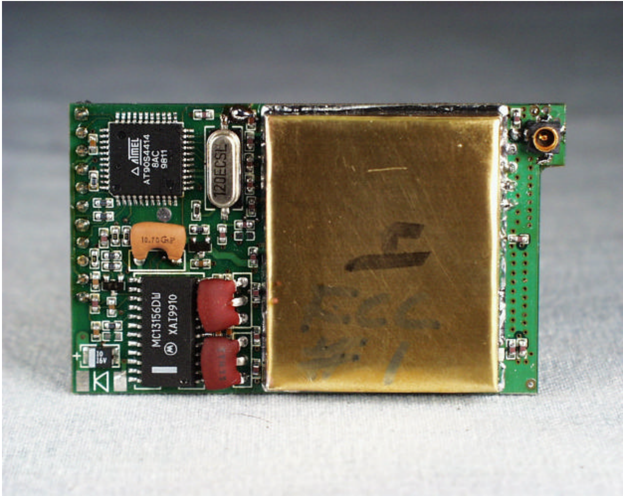
Front View of the Radio Board (with RF Can Installed)
