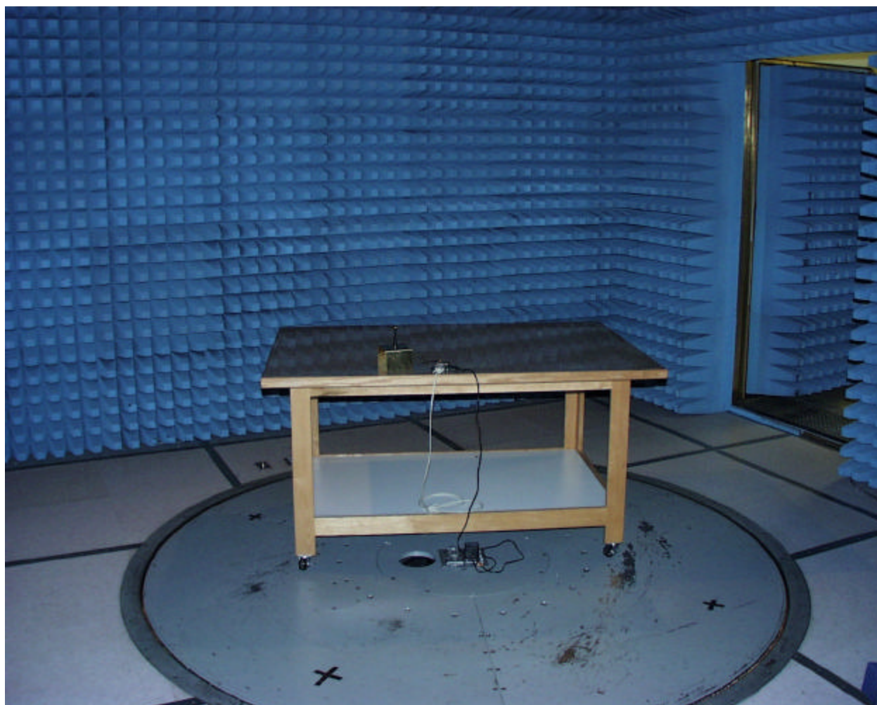
Worst case radiated emissions (Astron Monopole antenna)
