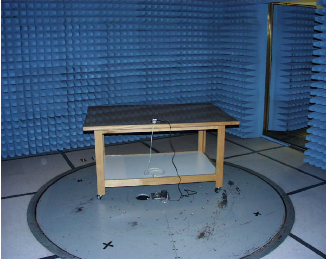
Worst case radiated emissions (Small Dipole antenna)
