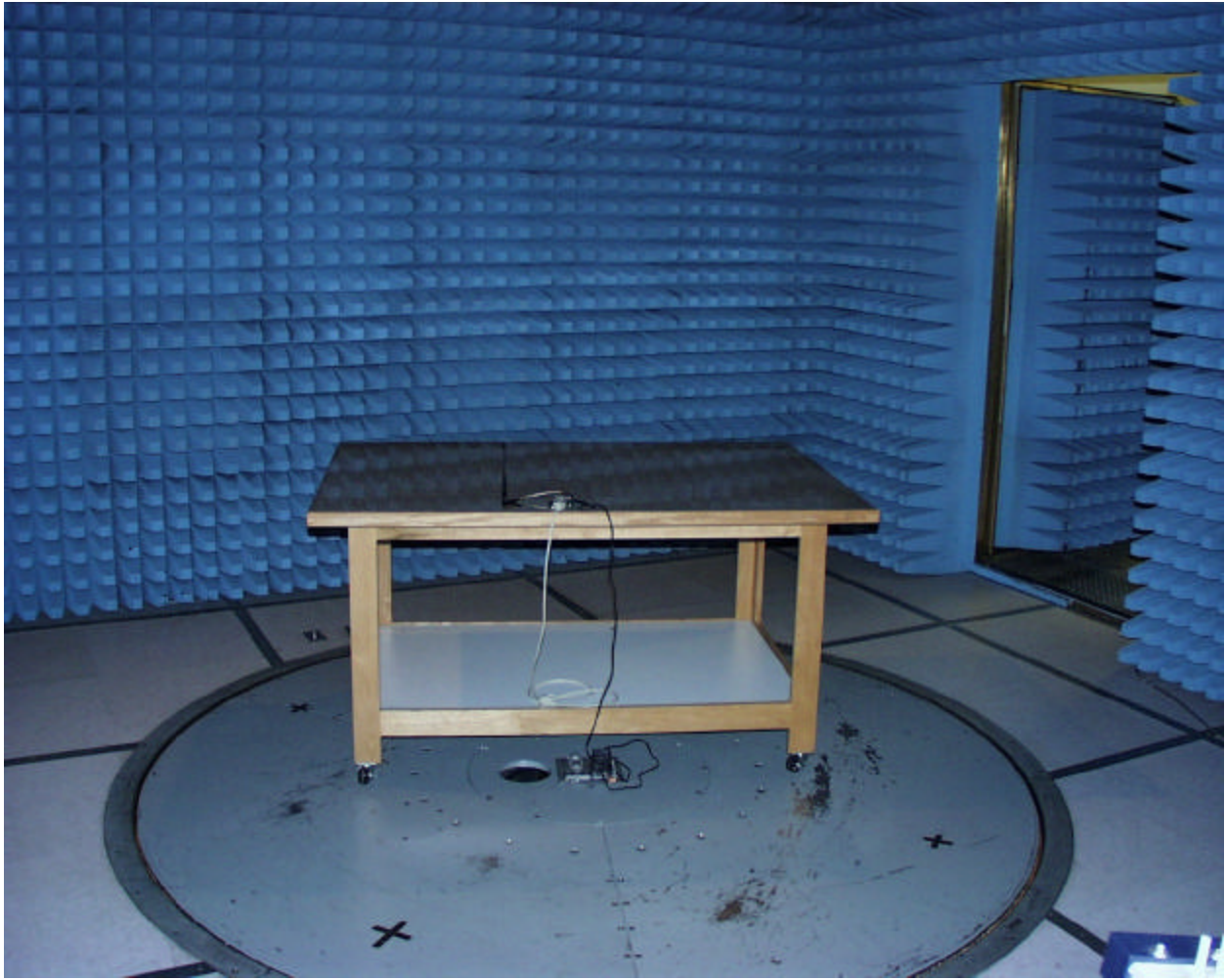
Worst case radiated emissions (Astron Dipole antenna)
