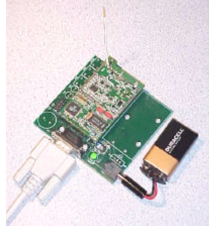
Figure 1– Demo Kit
