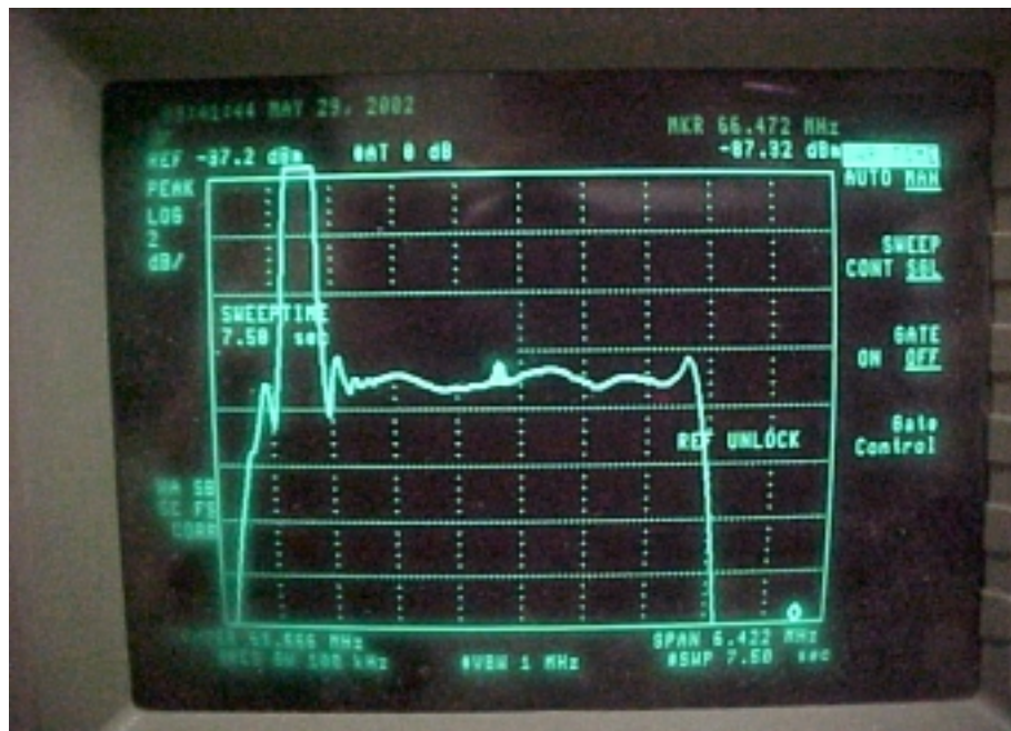
Figure 4-3. Graph of Detected Video Frequency Response
