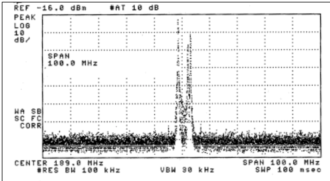
Figure 4-9. Products Above the 70 dB Noise Floor of the Spectrum Analyzer (One of Two)
