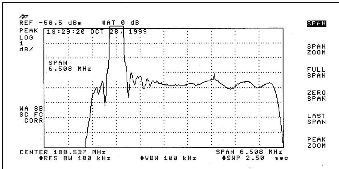
Figure 4-3. Graph of Detected Video Frequency Response
