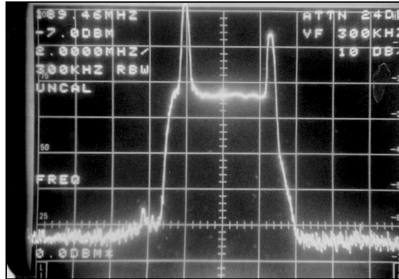
Figure 4-7. Channel Occupied Bandwidth
