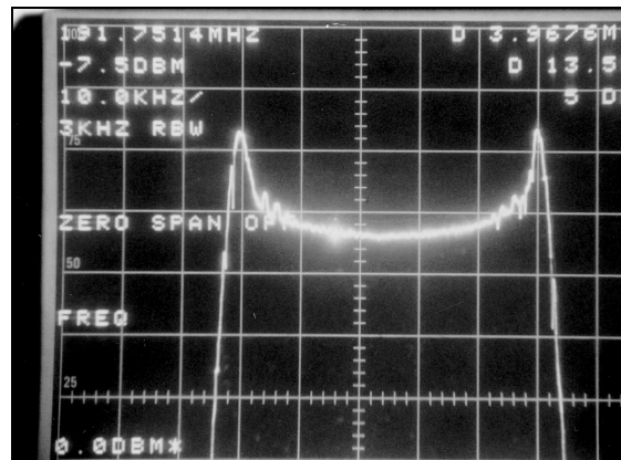
Figure 4-8. Aural Carrier Occupied Bandwidth
