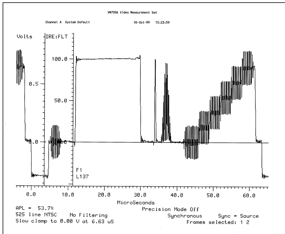
Figure 4-2. Substantially Linear Transfer Characteristics of the Transmitter as a Demodulated Video Waveform
