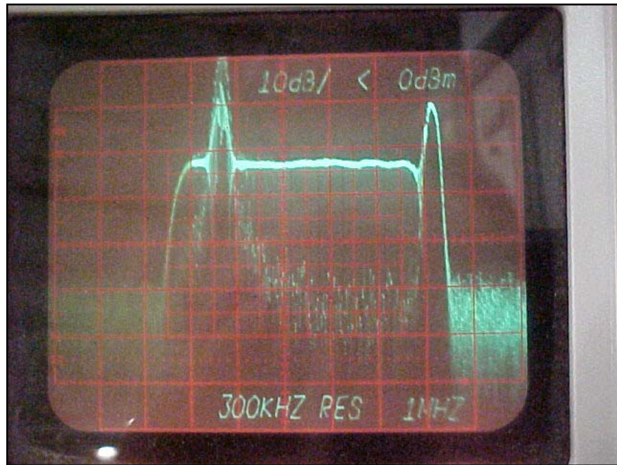
Figure 4-7. Channel-Occupied Bandwidth
