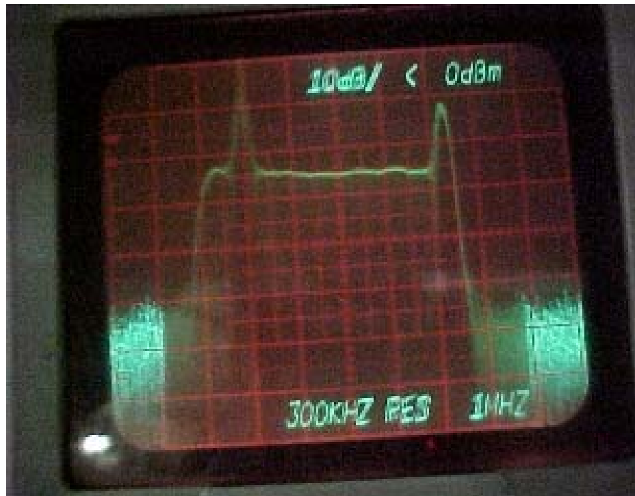
Figure 4-7. Channel-Occupied Bandwidth
