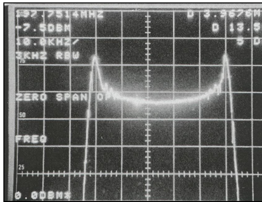
Figure 4-7. Aural Carrier Occupied Bandwidth
