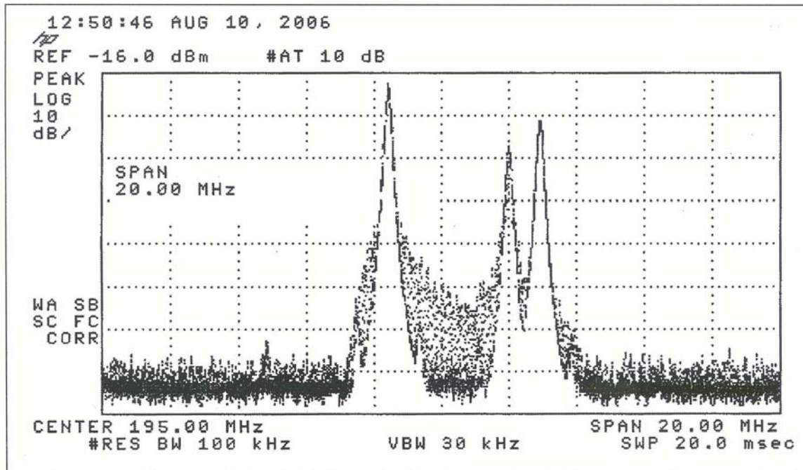
Figure 4-9. Products Above the 70 dB Noise Floor of the Spectrum Analyzer (Two of Two)
