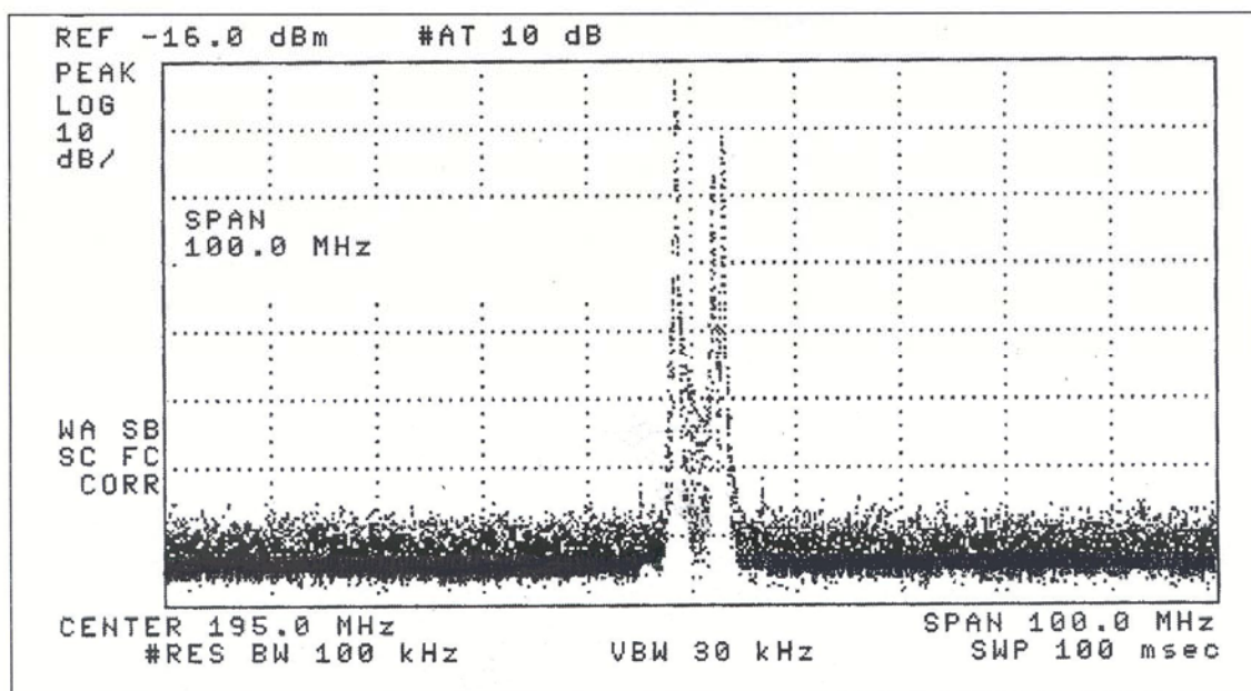
Figure 4-8. Products Above the 70 dB Noise Floor of the Spectrum Analyzer (One of Two)
