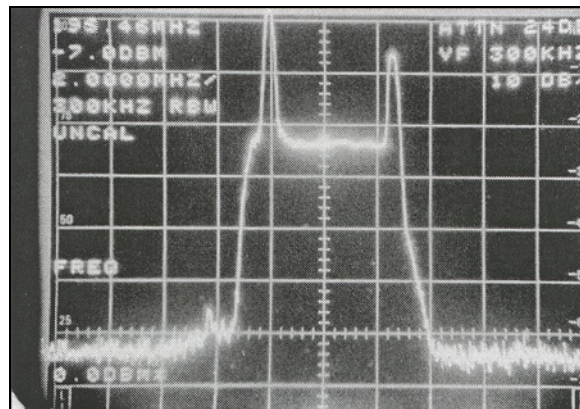
Figure 4-6. Channel Occupied Bandwidth
