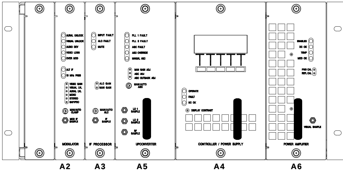
Figure 2-1: Transmitter Front View
