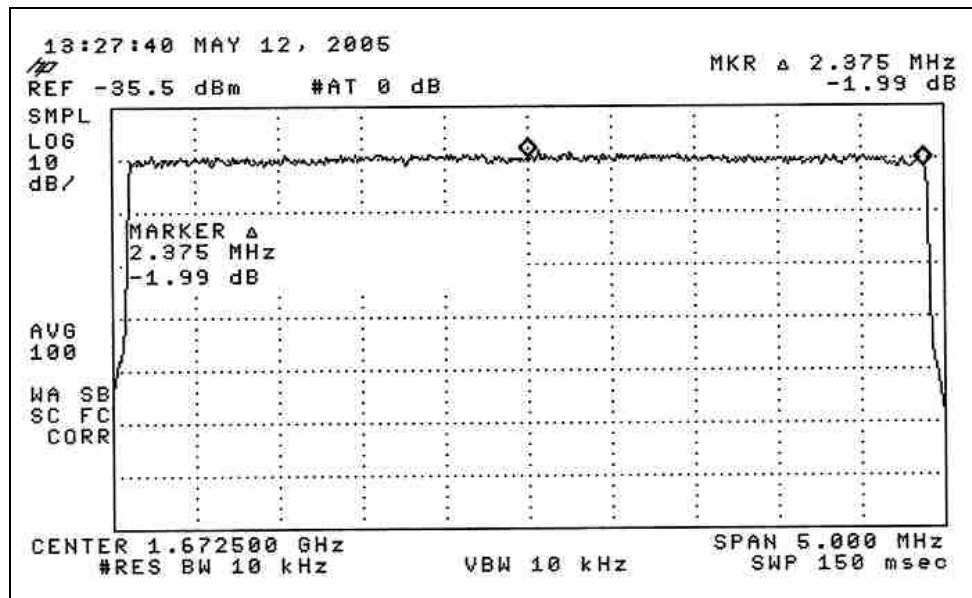
Figure 4-6. Channel Occupied Bandwidth (upper channel edge)
