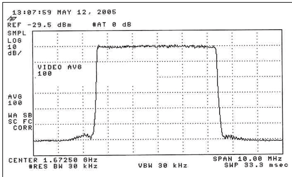
Figure 4-9. Conducted Spurious Emissions (after channel filter)
