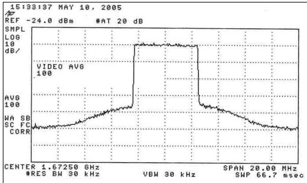
Figure 4-8. Conducted Spurious Emissions (before channel filter)
