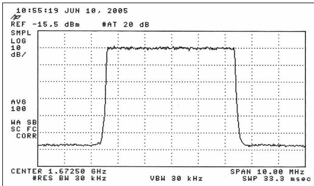
Figure 4-9. Conducted Spurious Emissions (after channel filter)
