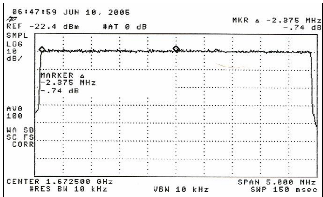
Figure 4-5. Channel Occupied Bandwidth (lower channel edge)
