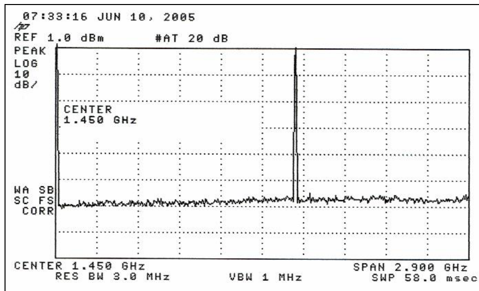
Figure 4-7. Products Above the -57 dB Noise Floor of the Spectrum Analyzer (2.900 GHz Span)
