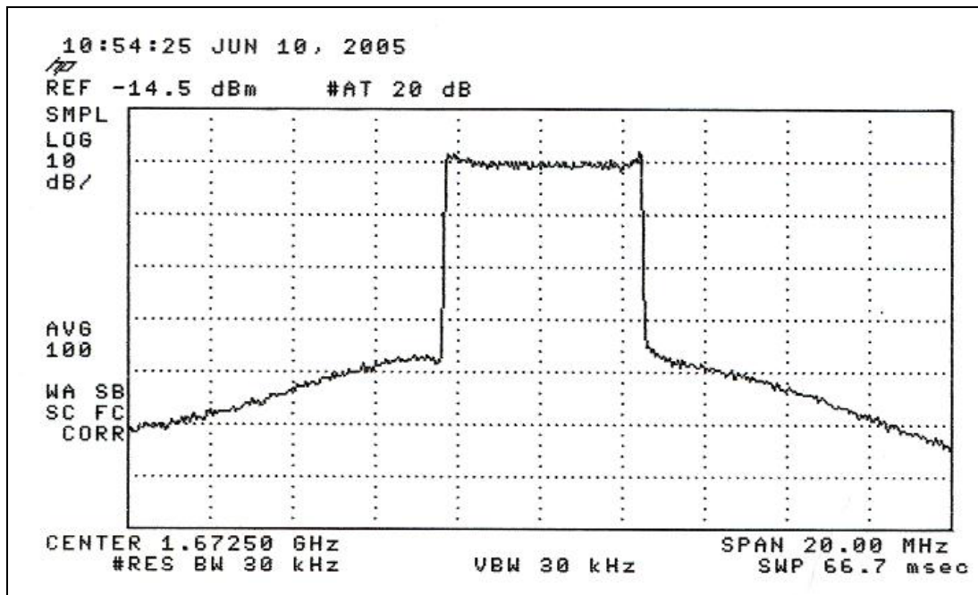
Figure 4-8. Conducted Spurious Emissions (before channel filter)
