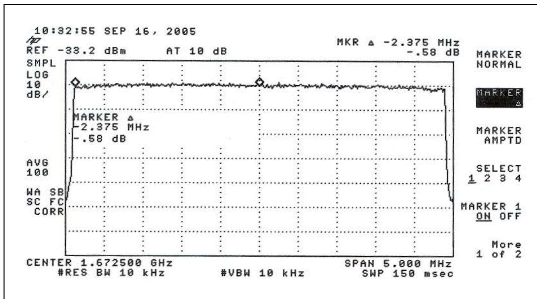
Figure 4-5. Channel Occupied Bandwidth (lower channel edge)
