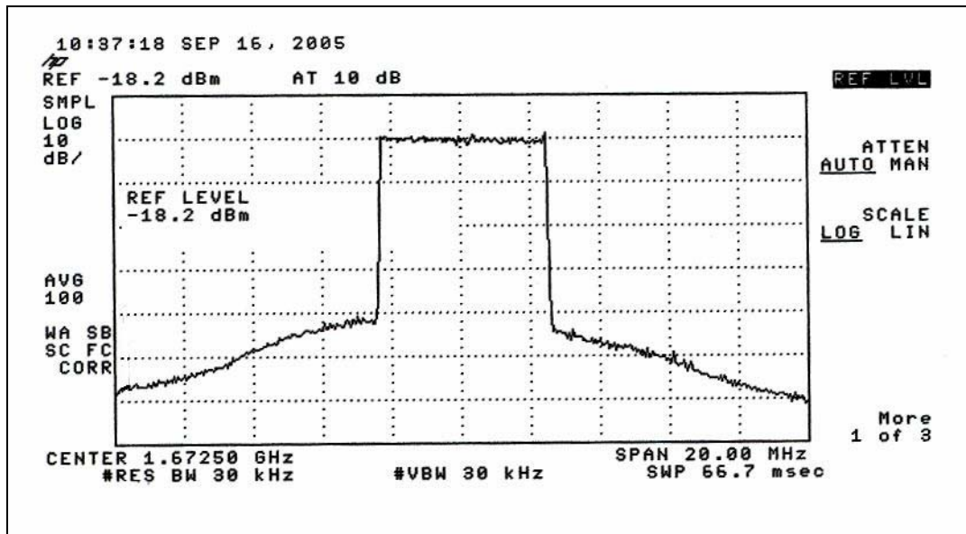
Figure 4-8. Conducted Spurious Emissions (before channel filter)
