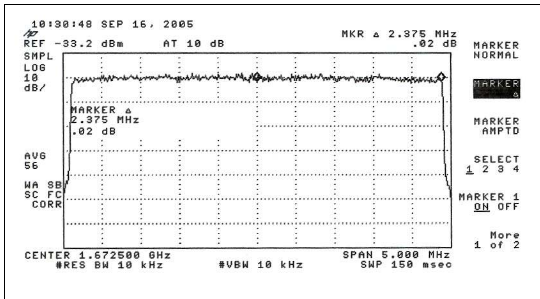
Figure 4-6. Channel Occupied Bandwidth (upper channel edge)
