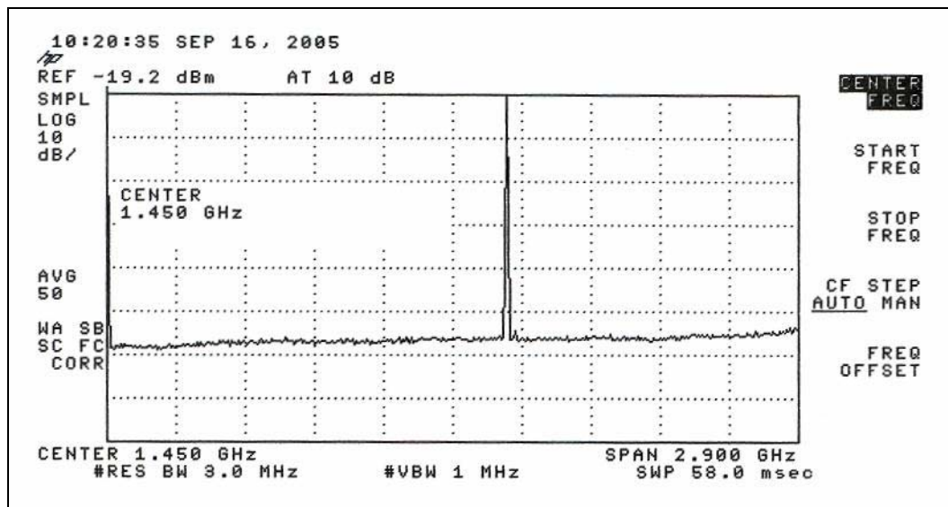
Figure 4-7. Products Above the -56 dB Noise Floor of the Spectrum Analyzer (2.900 GHz Span)
