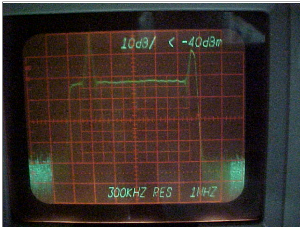
Figure 4-7. Channel-Occupied Bandwidth
