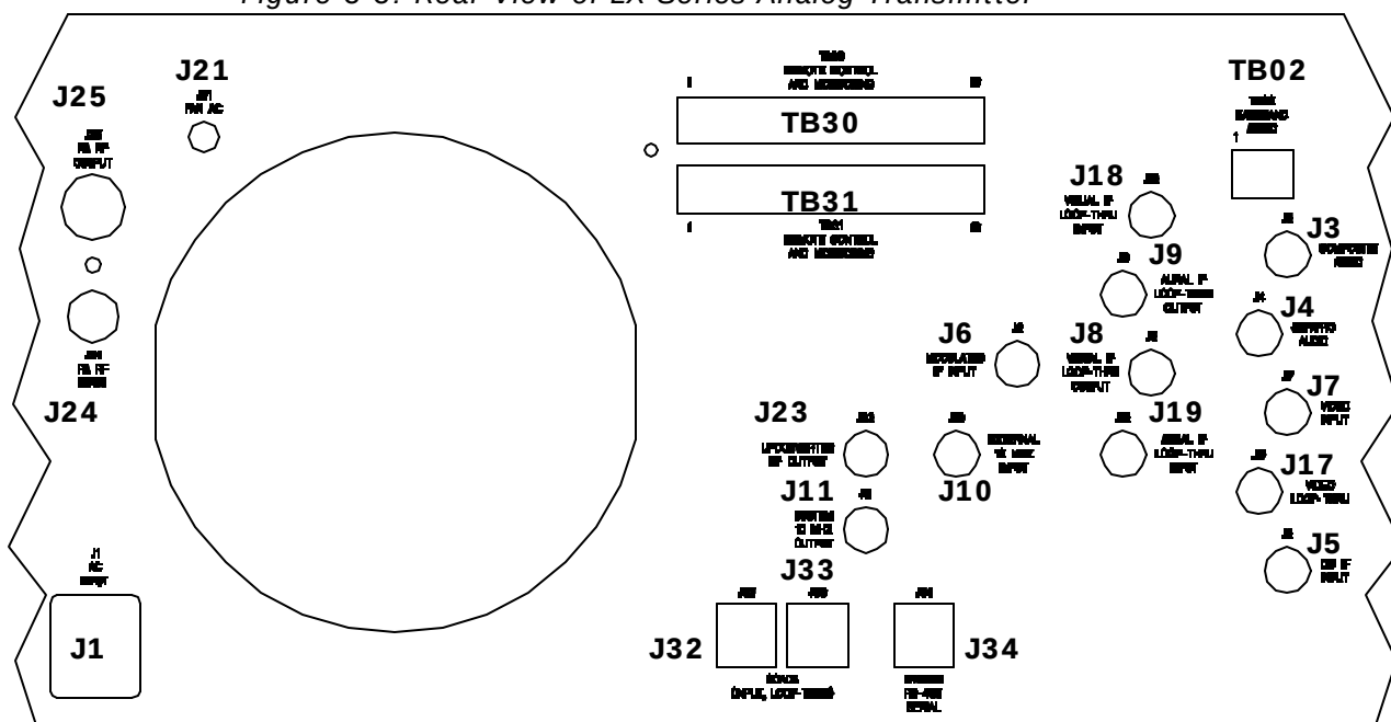
Figure 3-3: Rear View of LX Series Analog Transmitter
