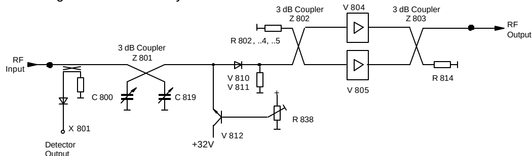
Figure 4-1: 40 Watt UHF Amplifier Module
