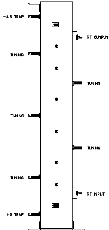
Figure 5-2. Bandpass Filter
