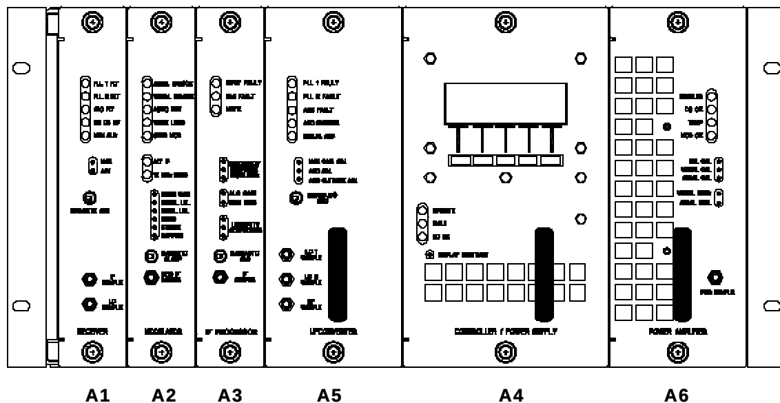
Figure 2-1: Exciter/Driver Front View
