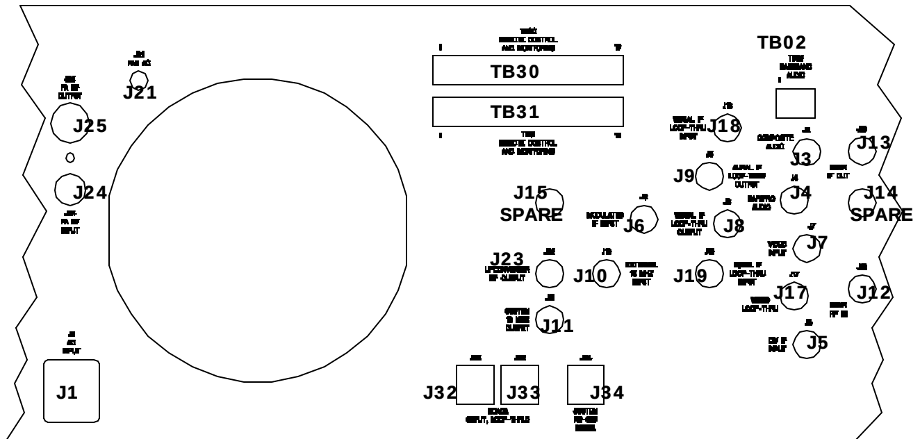
Figure 3-4: Rear View of LX Series Analog Transmitter
