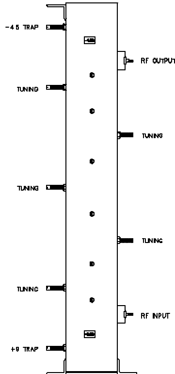
Figure 5-2. Bandpass Filter
