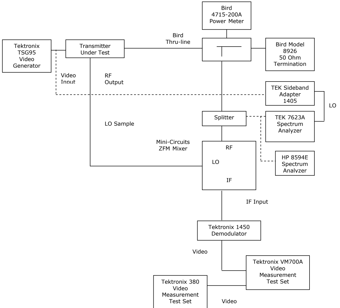
Figure 4-1. Test Equipment Setup for RF Power Measurements
