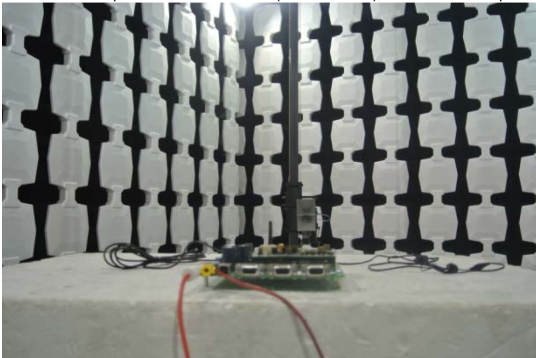
Radiated Spurious Measurement (Above 1GHz), EIRP Test Setup
