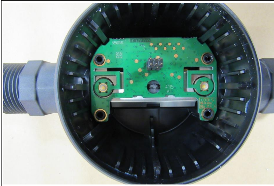
EUT LOWER PCB TOP IN HAUSING
