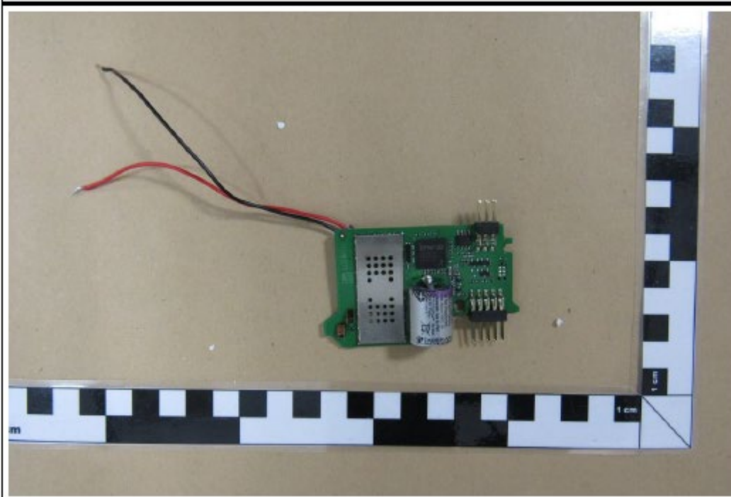
FlowIQ 3250 RF PCB
