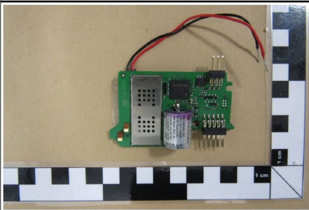
FlowIQ 2250 RF-PCB
