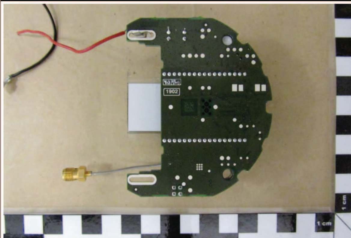
EUT, 55501810 conducted sample bottom view
