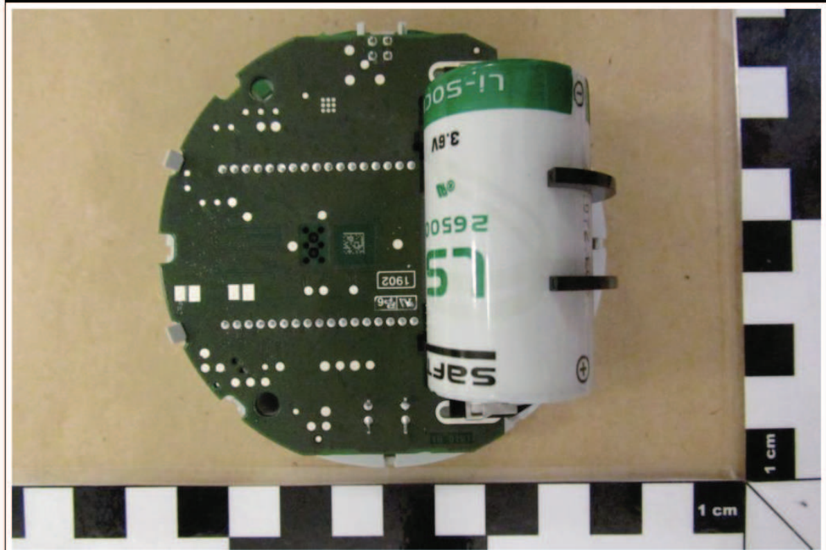
PCB, 55501810 assembly with battery bottom view
