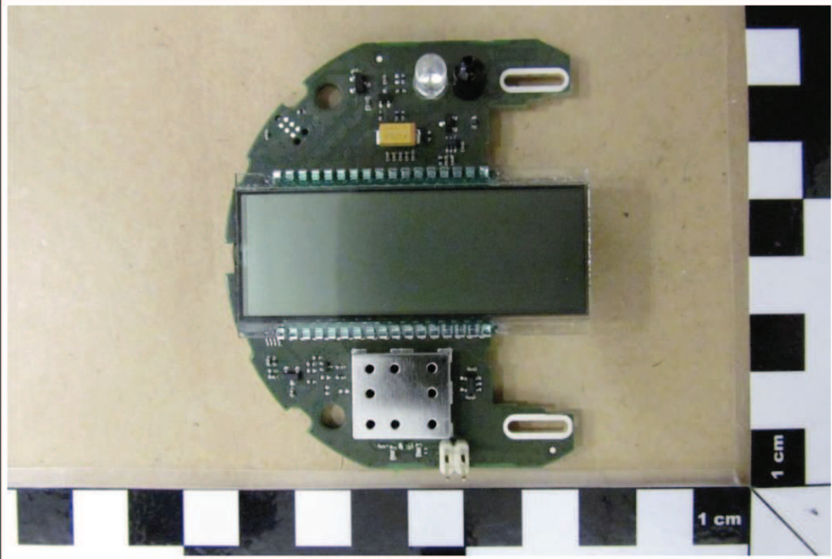
PCB, 55501810 radiated_sample
