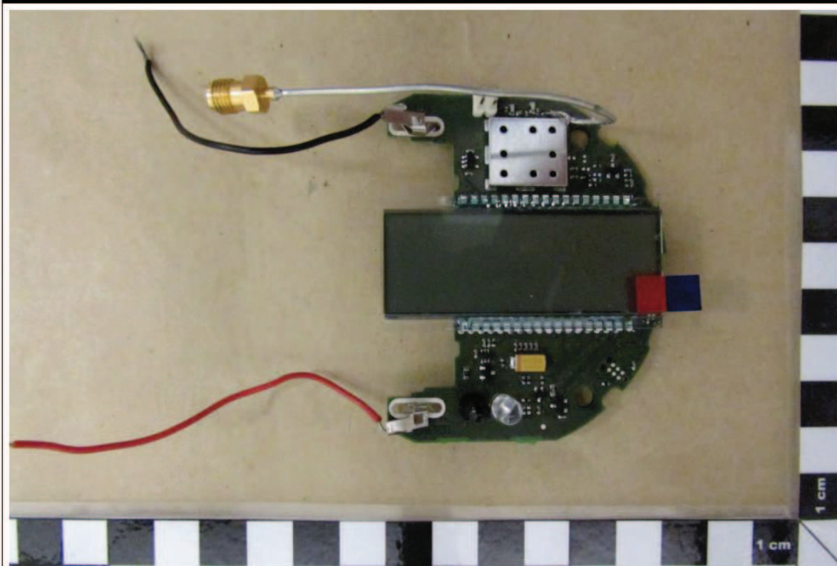
EUT, 55501810 conducted sample top view
