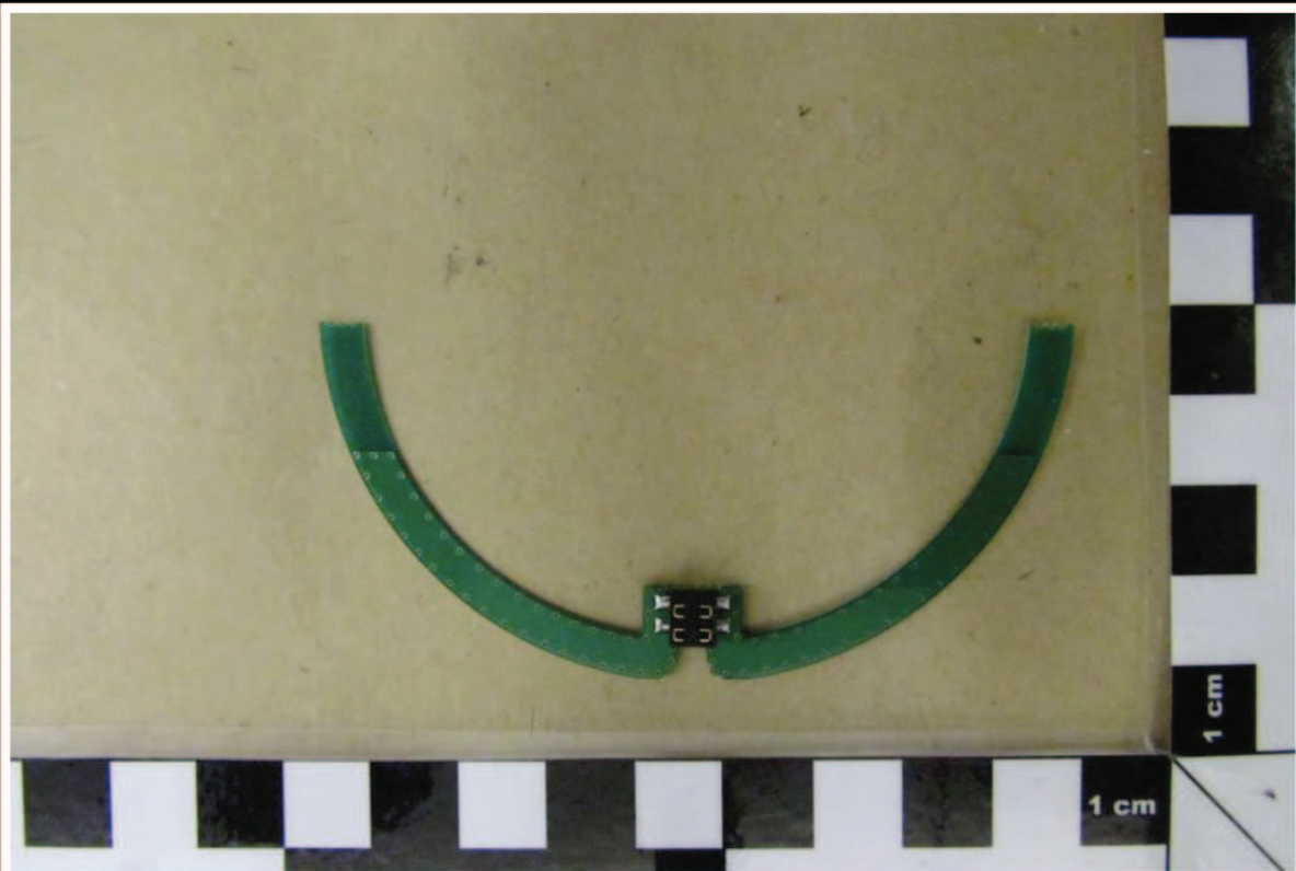
PCB, 55501350 antenna pcb
