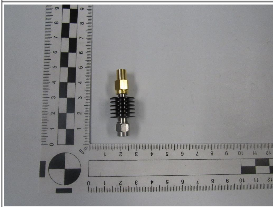
10 dB attenuator with 50 Ohm load
