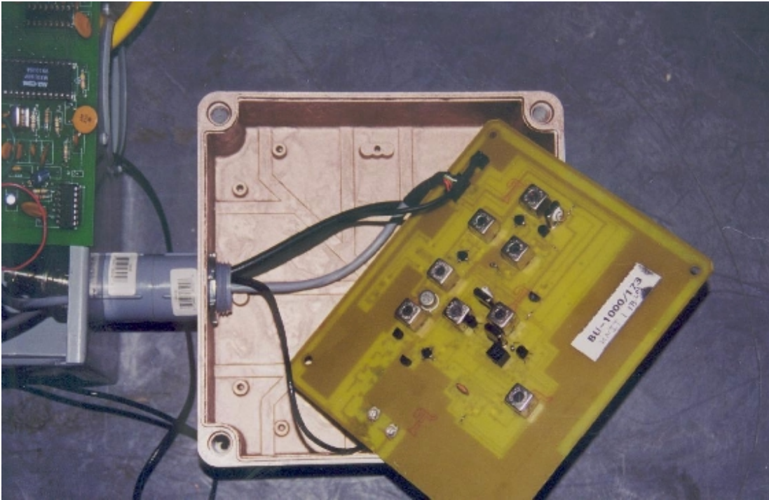
PHOTOGRAPH 1 TOP VIEW OF BU-1000 DATA TRANSCEIVER BOARD
