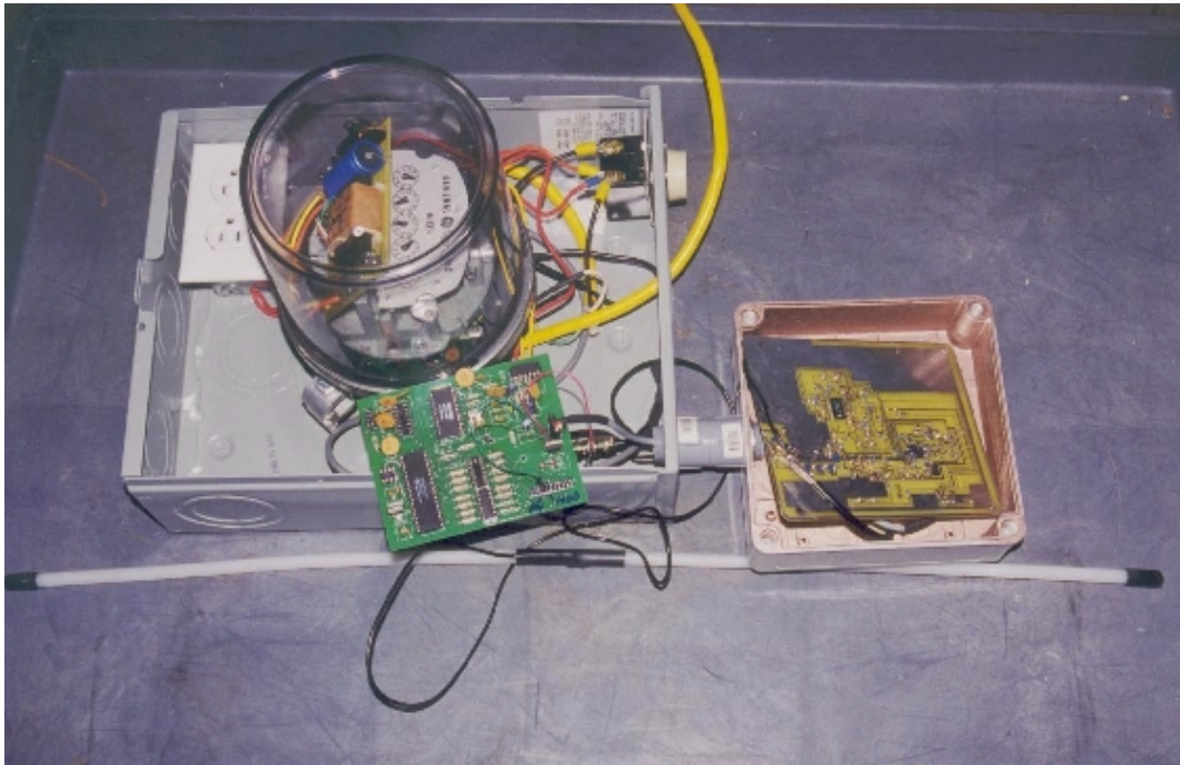
PHOTOGRAPH 3 VIEW OF BU-1000 AND SUPPORT EQUIPMENT: (MRU Board, Meter Dial Encoder, Enclosure and 173 MHz Dipole)
