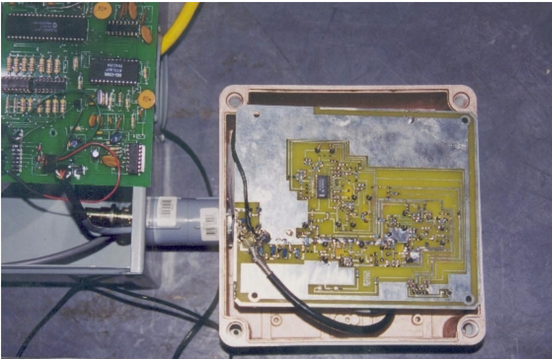
PHOTOGRAPH 2 BOTTOM VIEW OF BU-1000 DATA TRANSCEIVER BOARD
