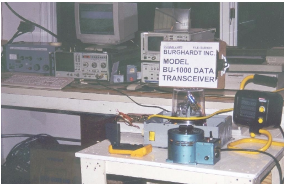
PHOTOGRAPH 9 RADIATED ELECTRIC FIELD EMISSIONS TESTS: 1 TO 5 GHz MEASUREMENTS
