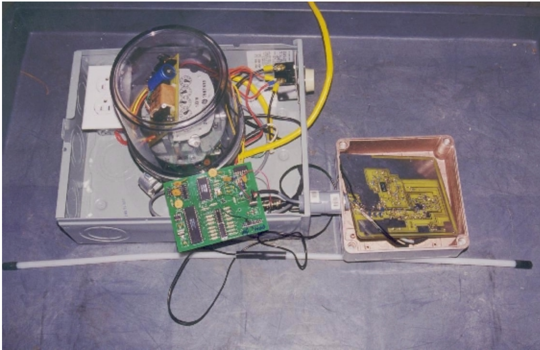
PHOTOGRAPH 3 VIEW OF BU-1000 AND SUPPORT EQUIPMENT: (MRU, Meter Dial Encoder, Enclosure and 173 MHz Dipole)
