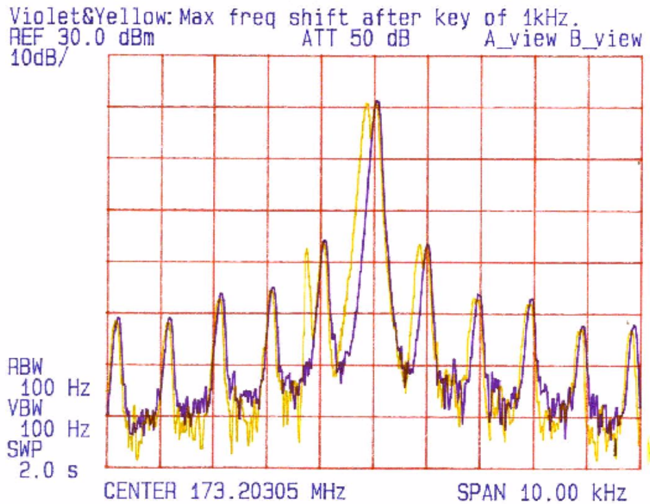
PLOT 11 FREQUENCY SHIFT AFTER KEYING OF 1kHz TEST SIGNAL FOR 173.2030 MHz
