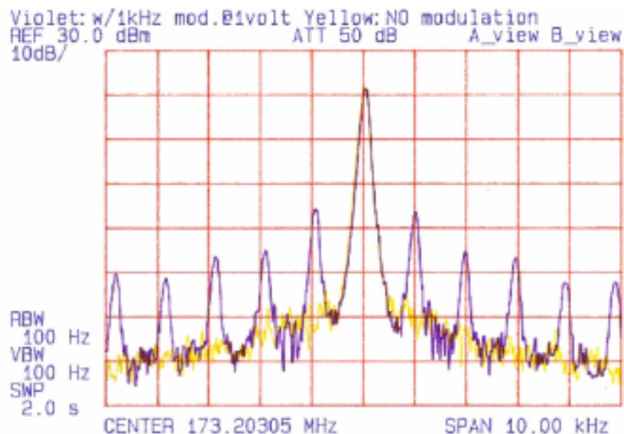
PLOT 10: 173.2030 MHz WITH & WITHOUT 1kHz TEST SIGNAL MODULATION
