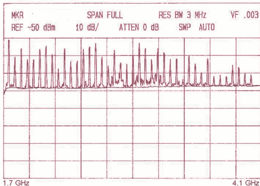
PLOT 9: RELATIVE LEVEL OF SPURIOUS EMISSIONS @ ANTENNA TERMINALS FOR 173.39625 MHz
