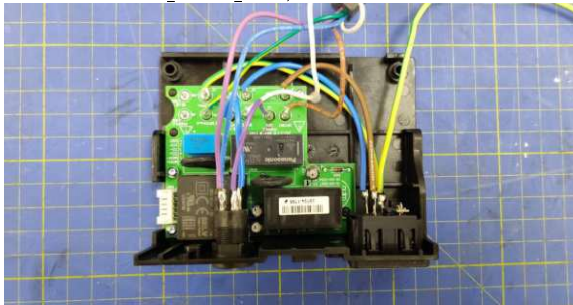
IMG_20250327_102138, EUP SMPS Module PCB
