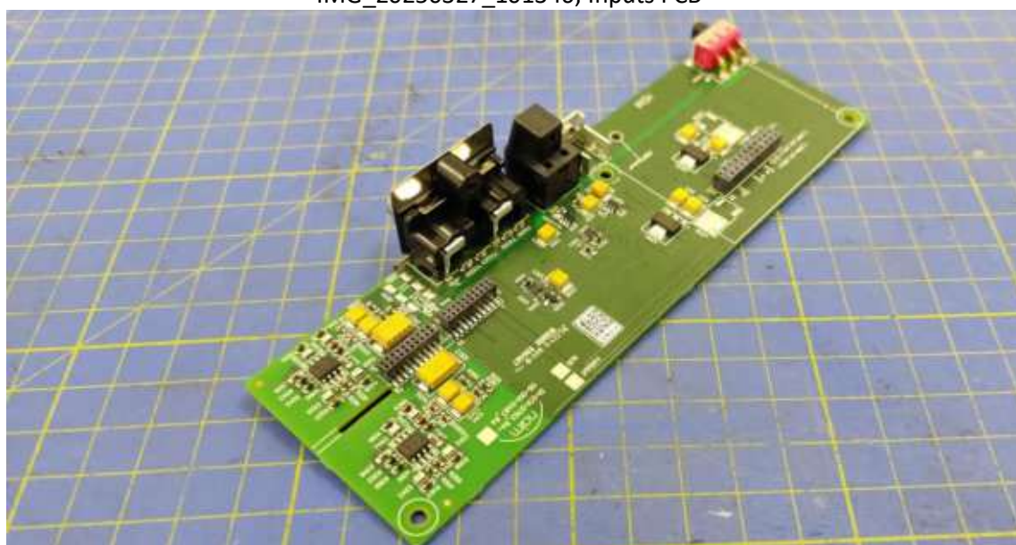
IMG_20250327_101346, Inputs PCB
