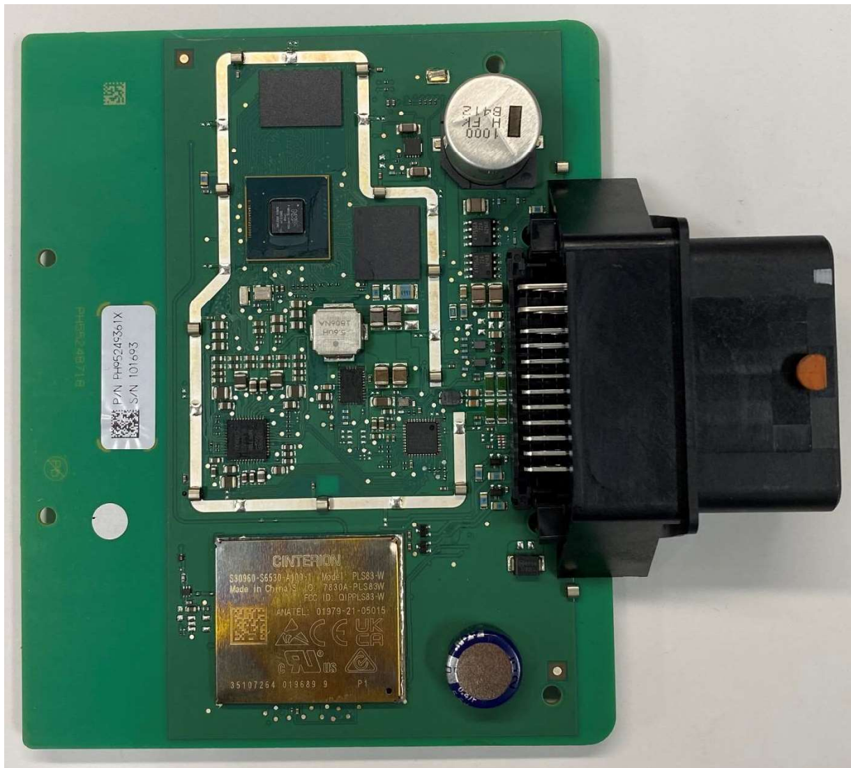
Top of main PCB
