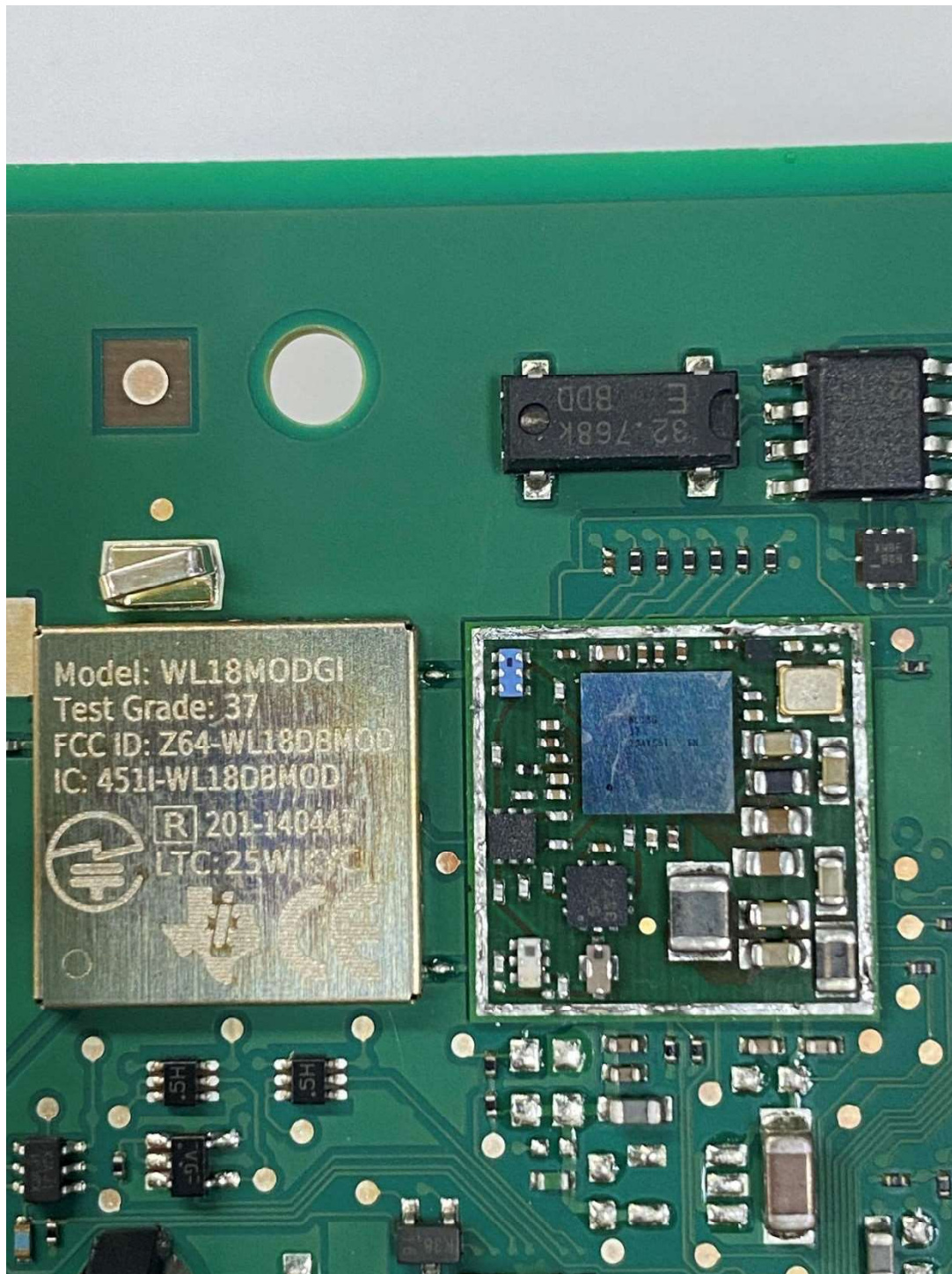
Wi-Fi PCB Close up
