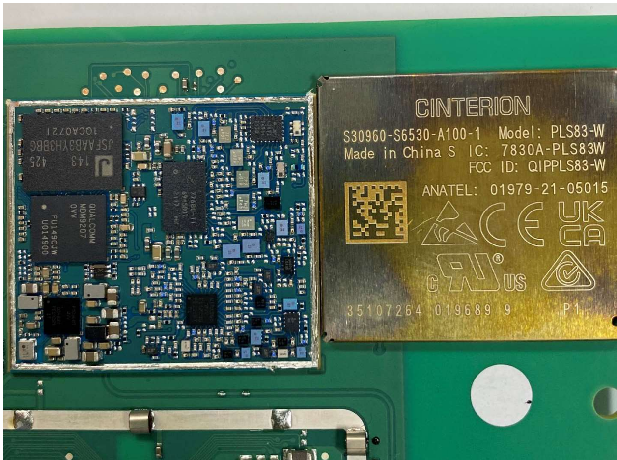
Cell module PCB close up
