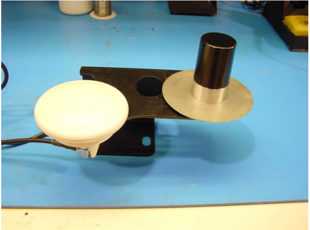
JDLink cell and GPS antennas with mounting bracket
