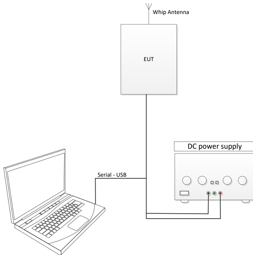
Figure 3.5-1: block diagram
