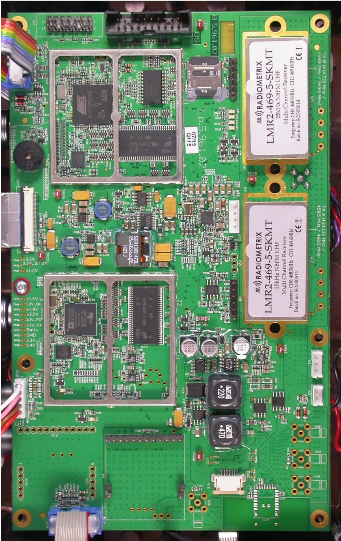
Main board top view
