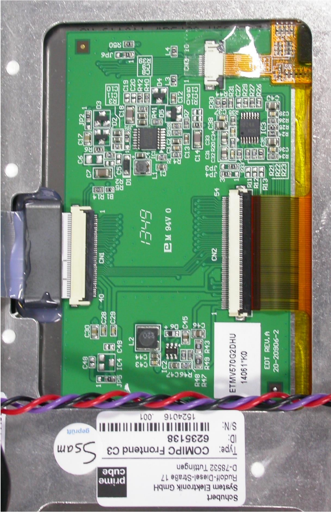
Display panel top view
