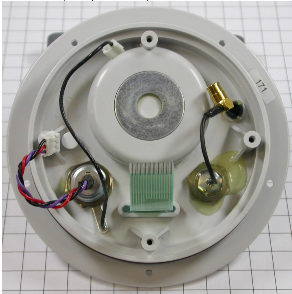
Top case (connector side) with removed mainboard
