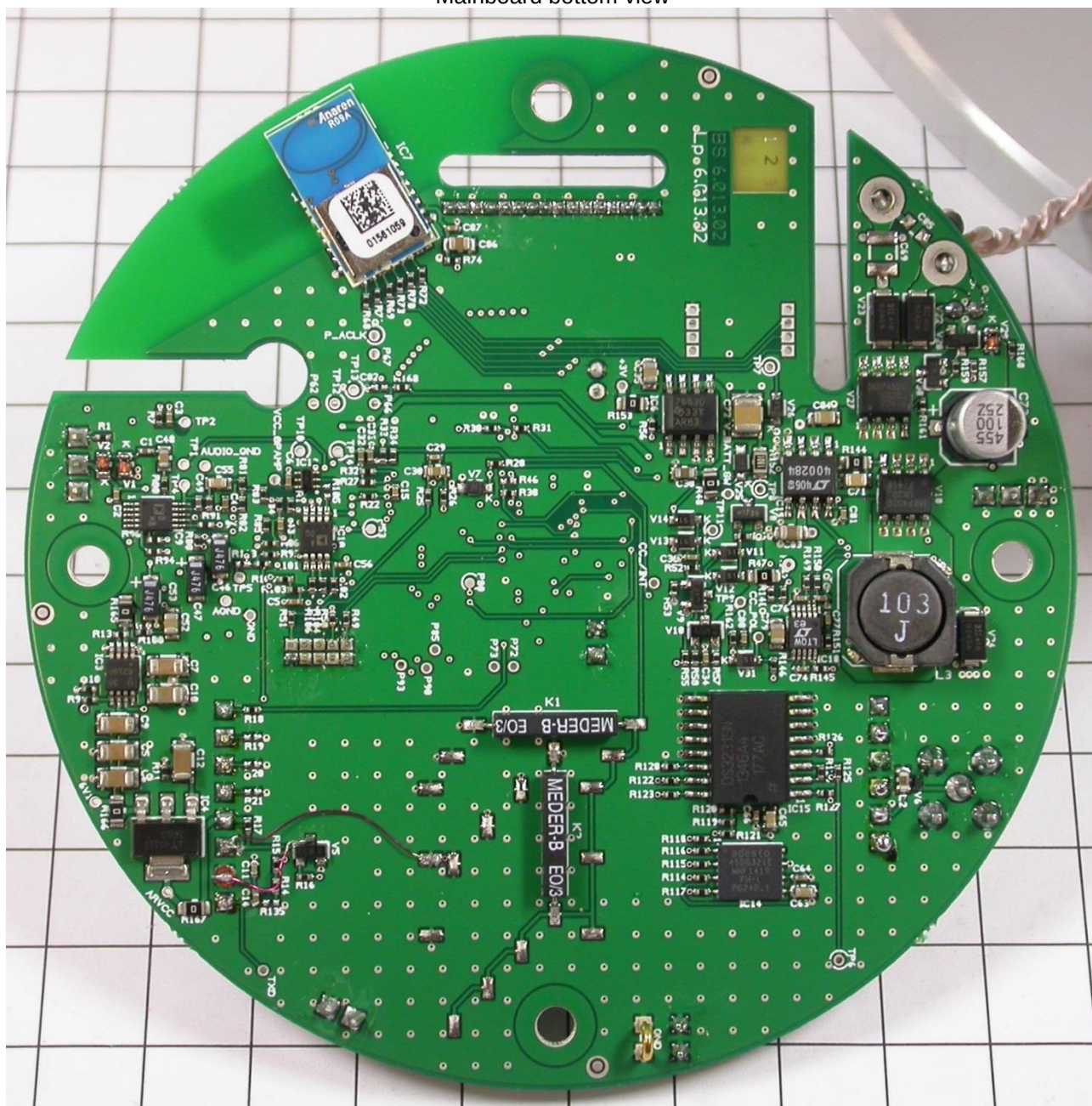
Mainboard bottom view
