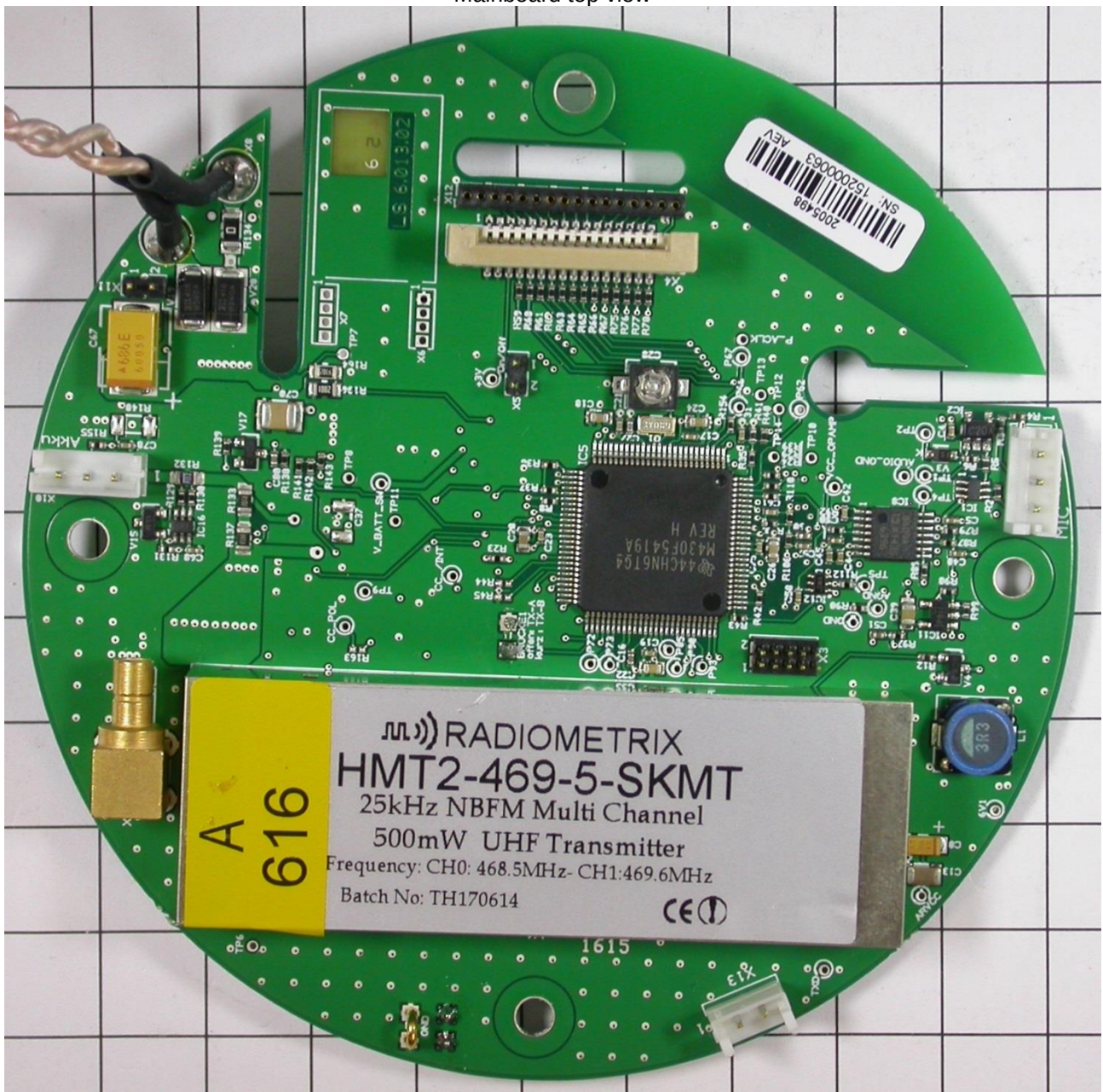
Mainboard top view
