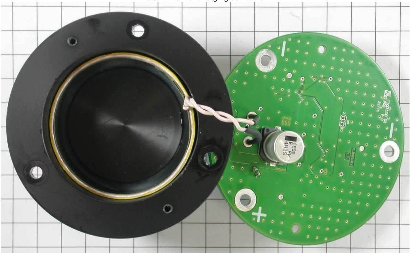
Bottom view of charging coil & PCB
