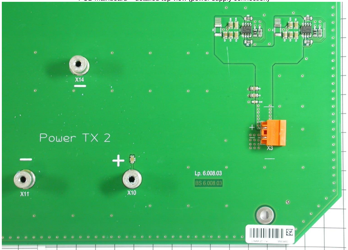
PCB mainboard – detailed top view (power supply connection)
