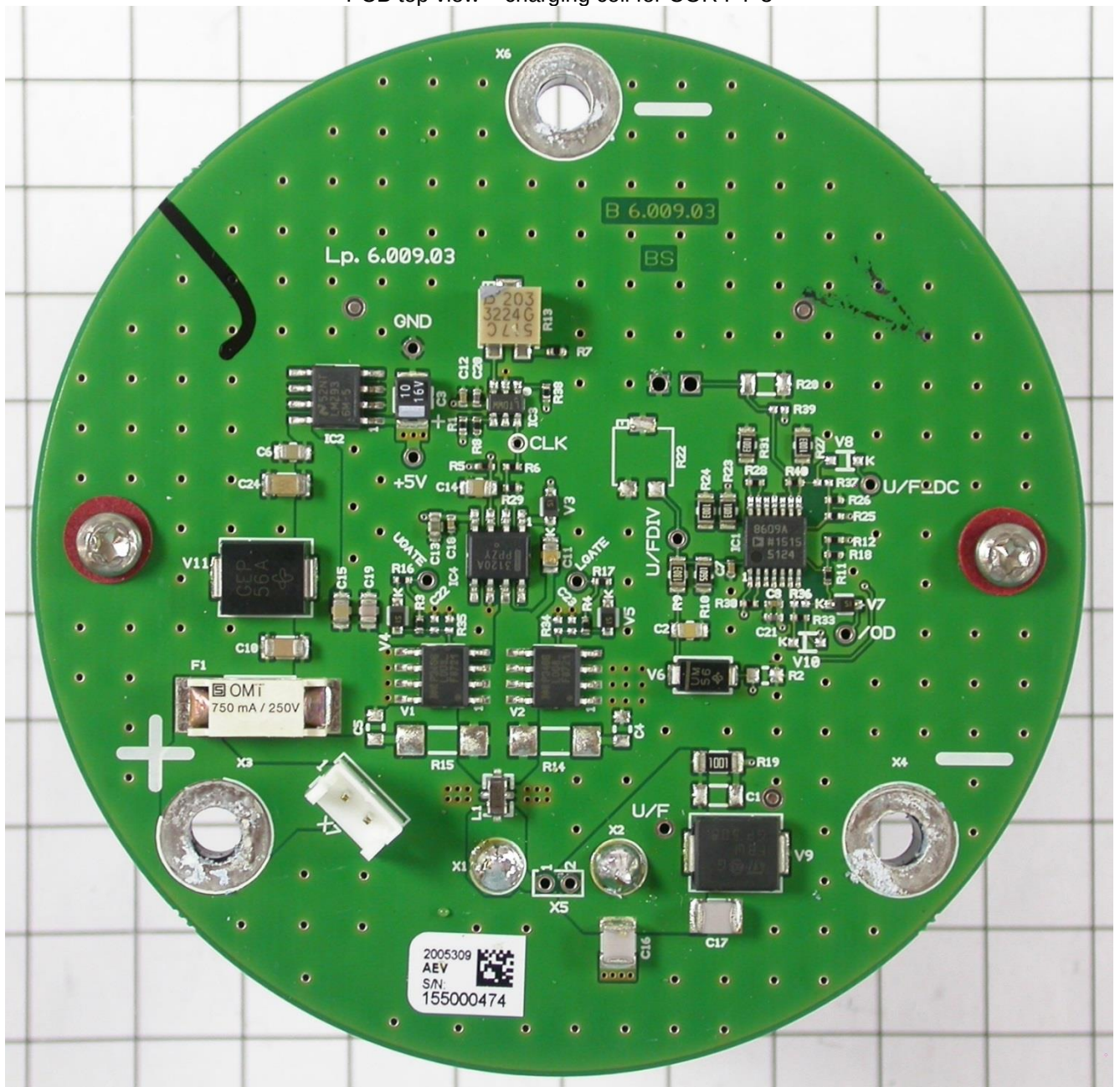
PCB top view – charging coil for COR PT-3
