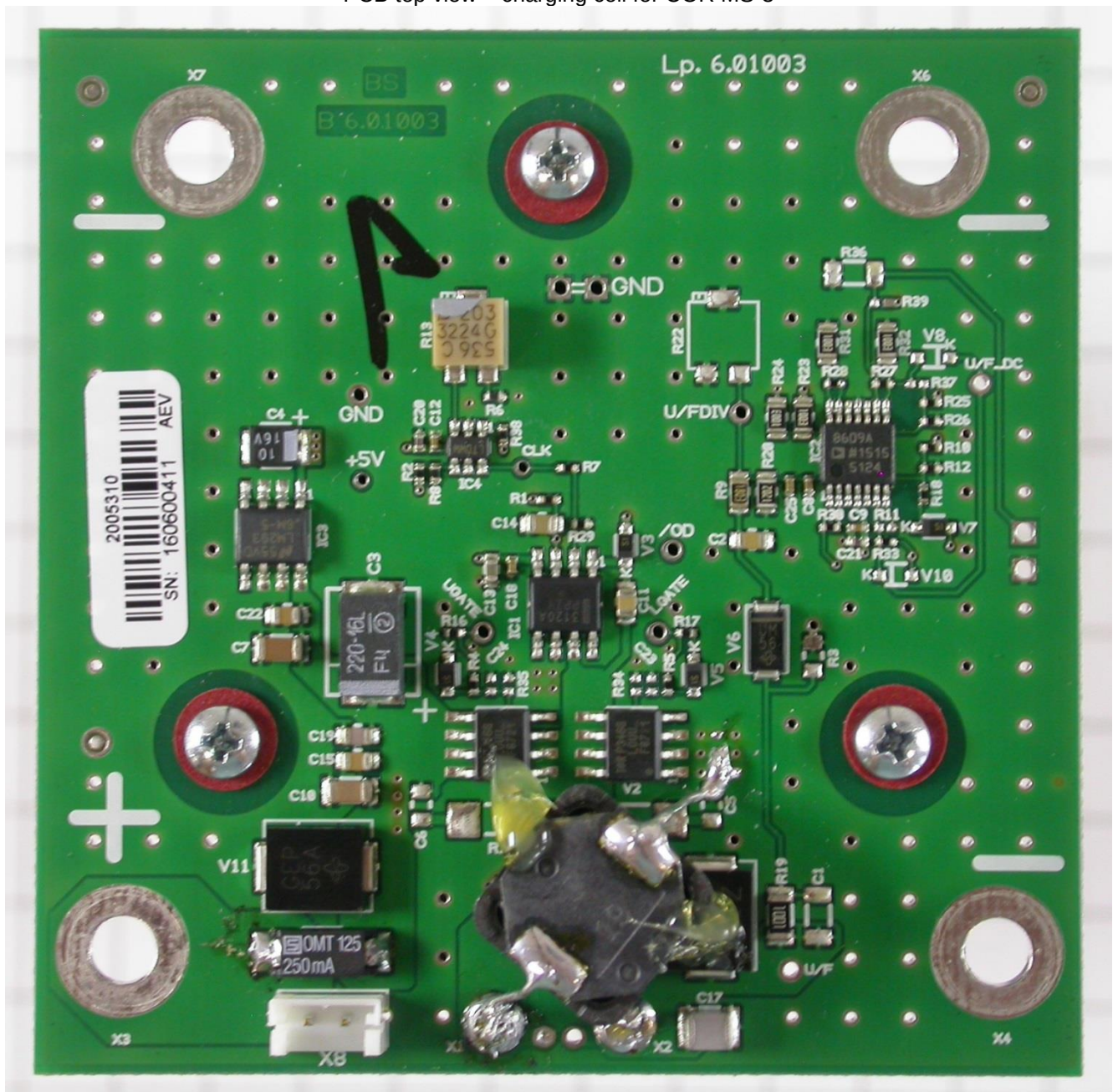
PCB top view – charging coil for COR MS-3
