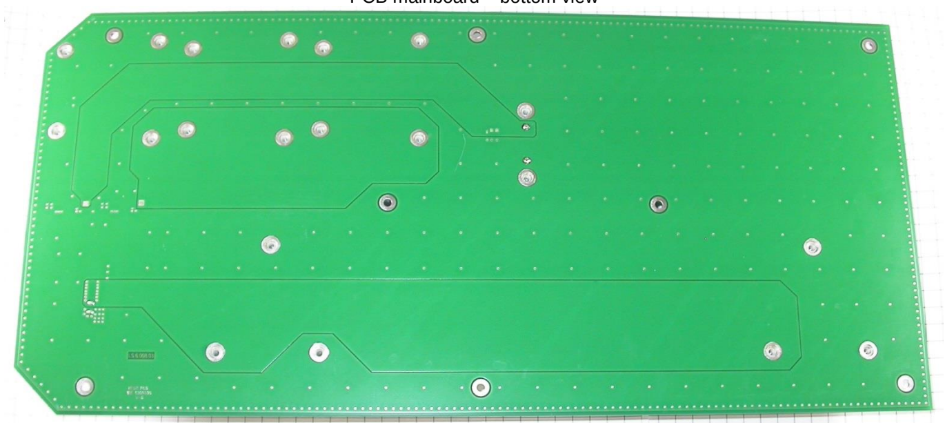
PCB mainboard – bottom view
