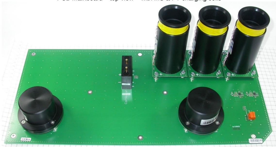
PCB mainboard – top view – with MS & PT charging coils
