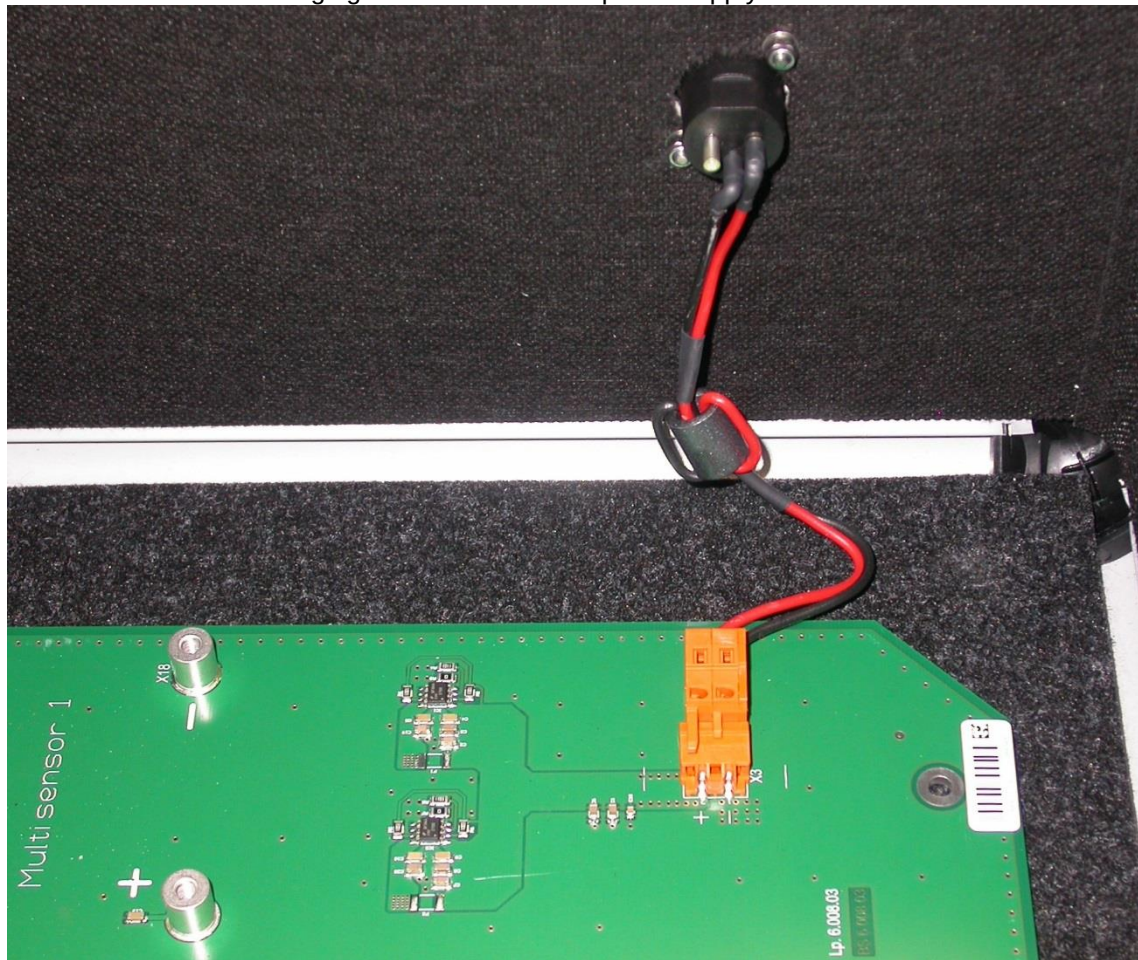
Charging box – inside view – power supply connection
