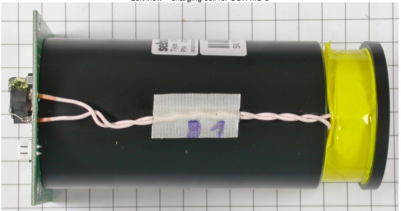
Left view – charging coil for COR MS-3
