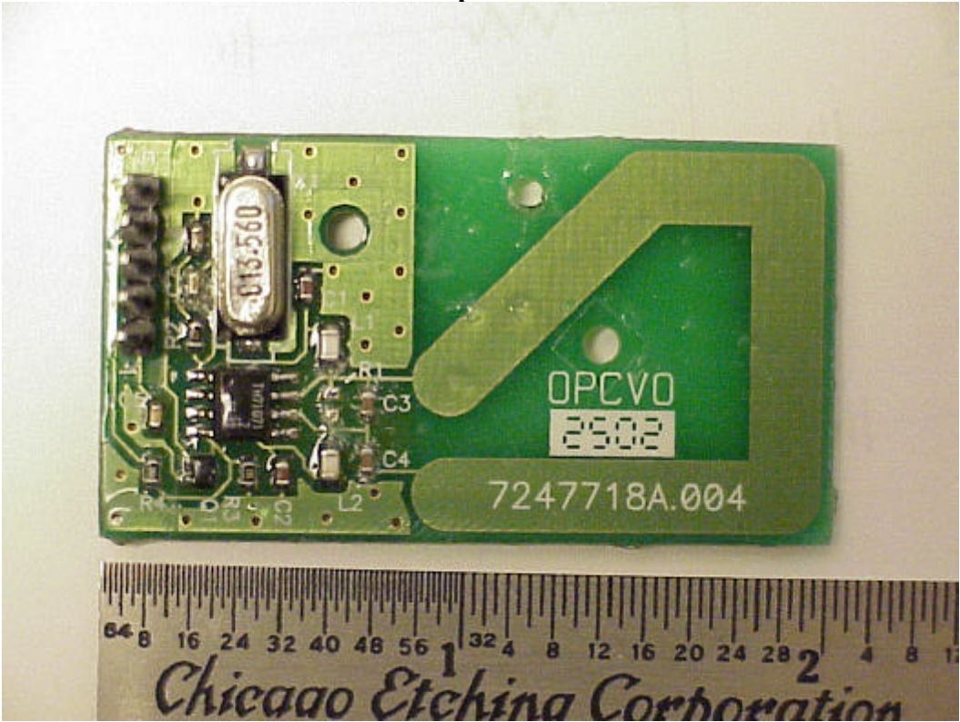
Top view
