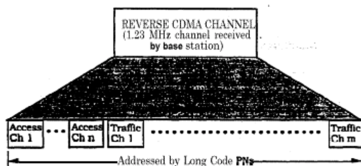
Figure 6.1.3.1-1. Example of Logical Reverse CDMA Channels Received at a Base Station
