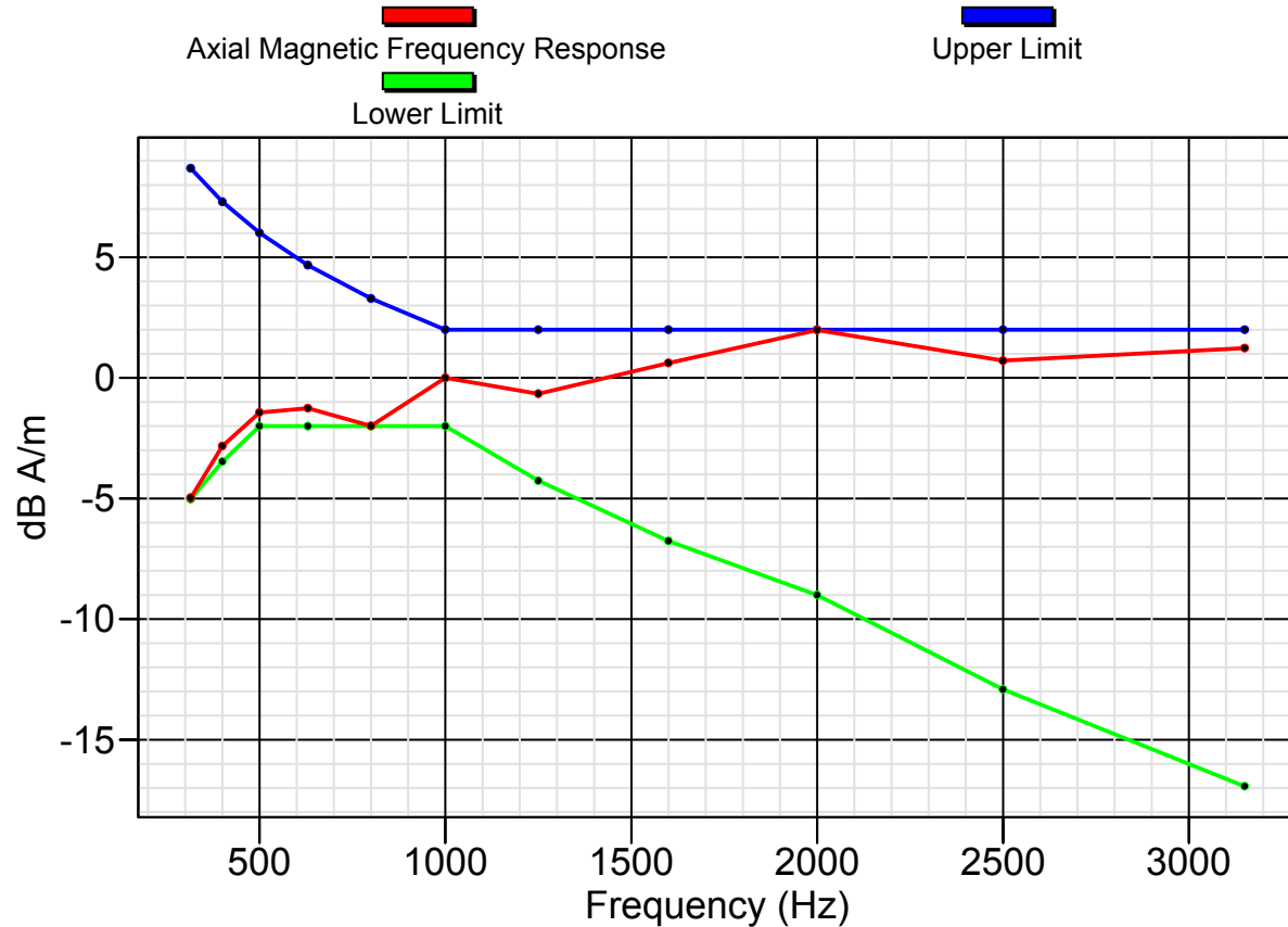
Frequency Response CDMA 1900
