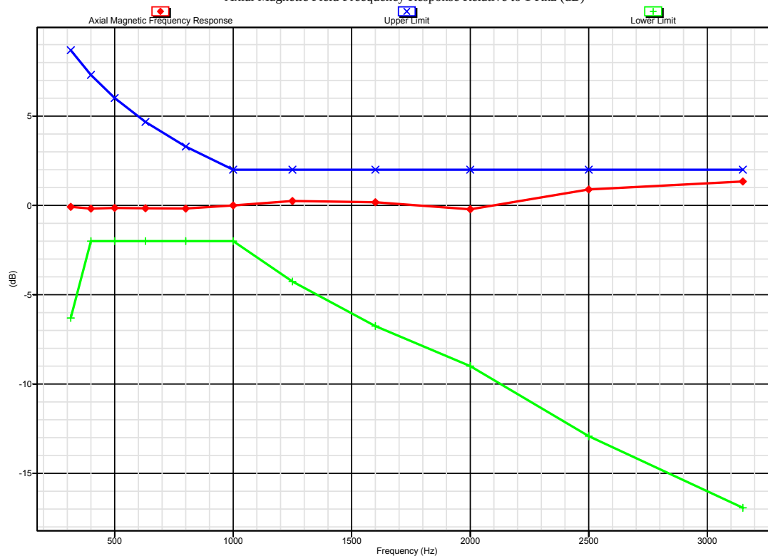
Axial Magnetic Field Freequency Response Relative to 1 KHz (dB)
