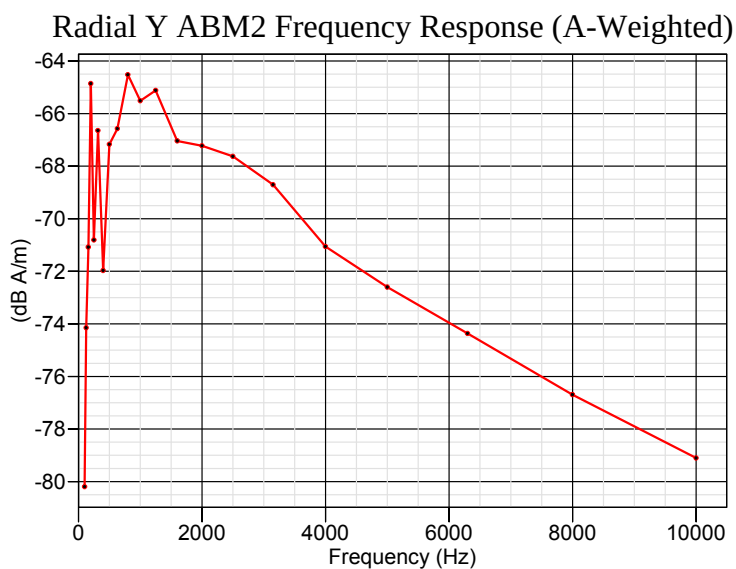
Radial Y ABM2 Frequency Response
