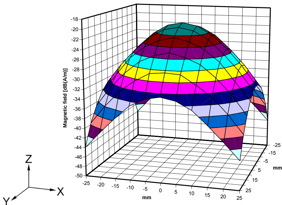
Distribution of magnetic field (axial component) at 5x5cm reference plane Input connector at -X
