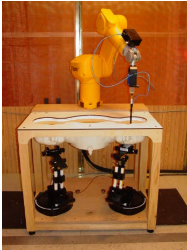
Figure 7.1 DASY 4 System
