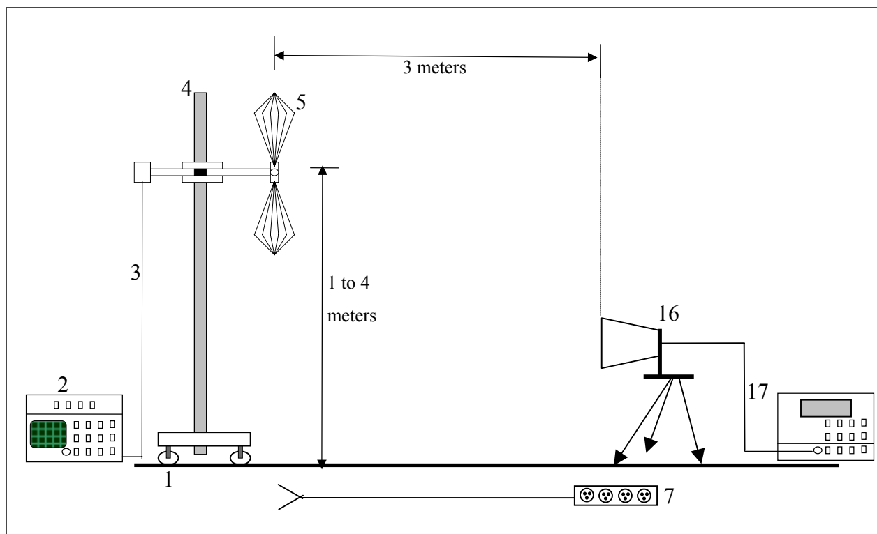
Figure 2. Substitution Method Test Setup Diagram
