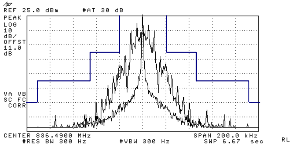
Figure 7-7 AMPS WIDEBAND
