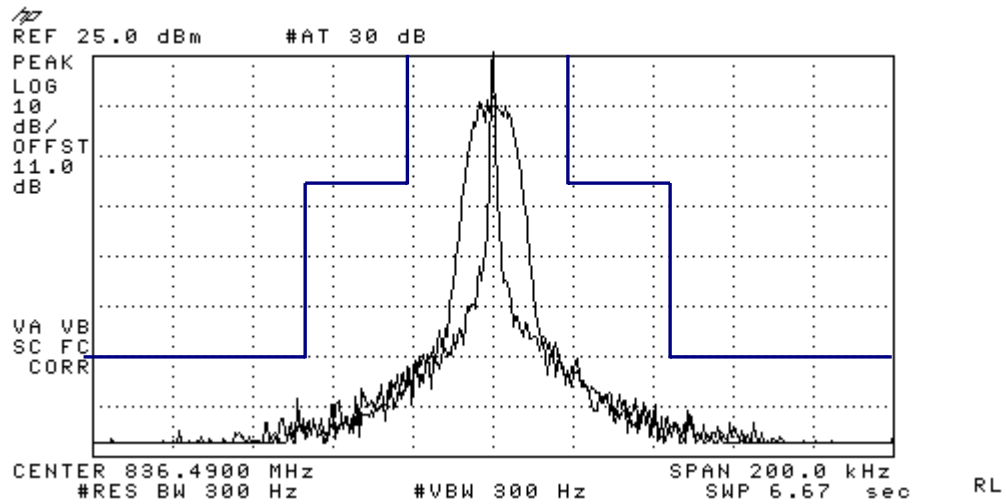
Figure 7-6 SAT + DTMF_9
