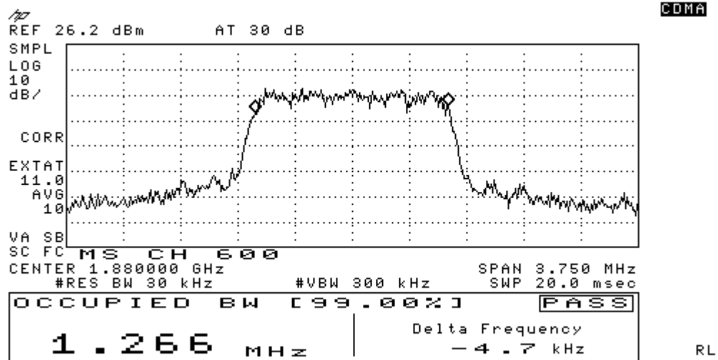
Figure 7-9 CDMA 1900 @ CH 600
