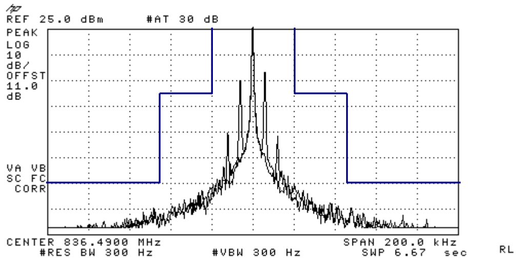
Figure 7-2 AMPS SAT
