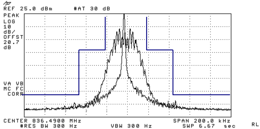
Figure 7-3 AMPS Voice + SAT
