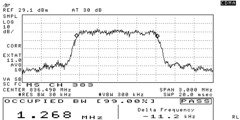
Figure 7-8 CDMA 800 @ CH 383
