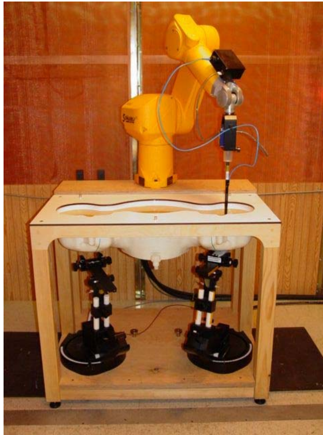
Figure 1. DASY 4 System
