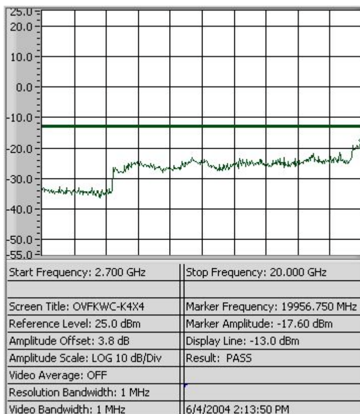
Figure 9-6b AMPS – Conducted Spurious Emission (CH 799)
