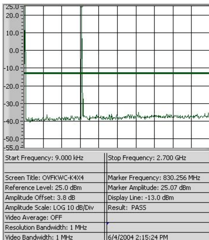
Figure 9-8a CDMA 800 – Conducted Spurious Emission (CH 1013)
