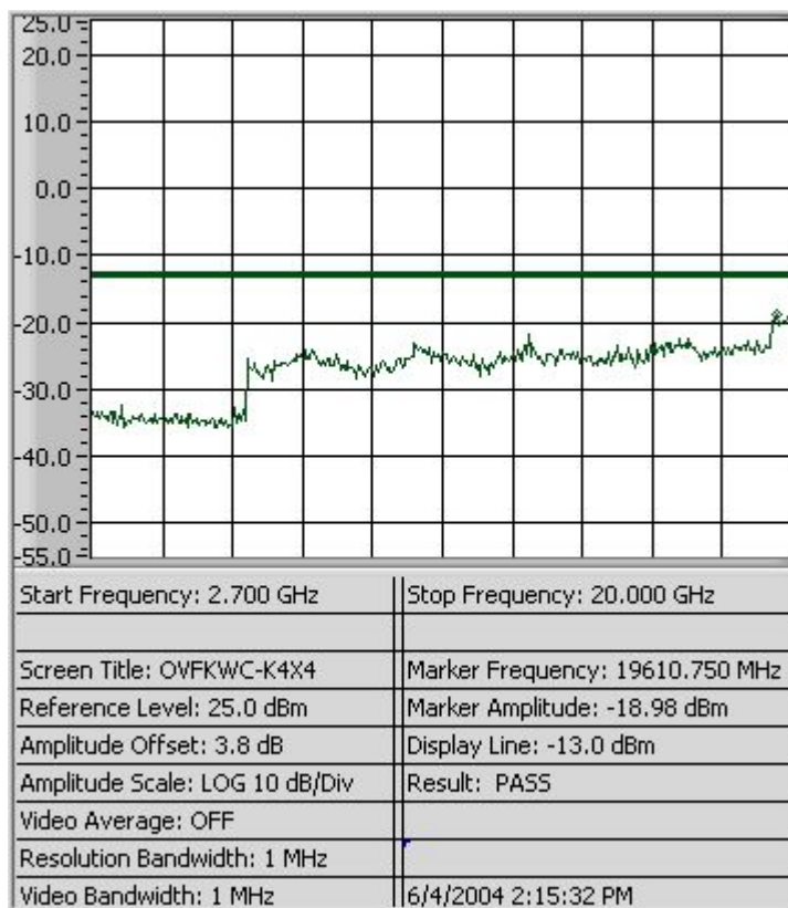
Figure 9-8b CDMA 800 – Conducted Spurious Emission (CH 1013)
