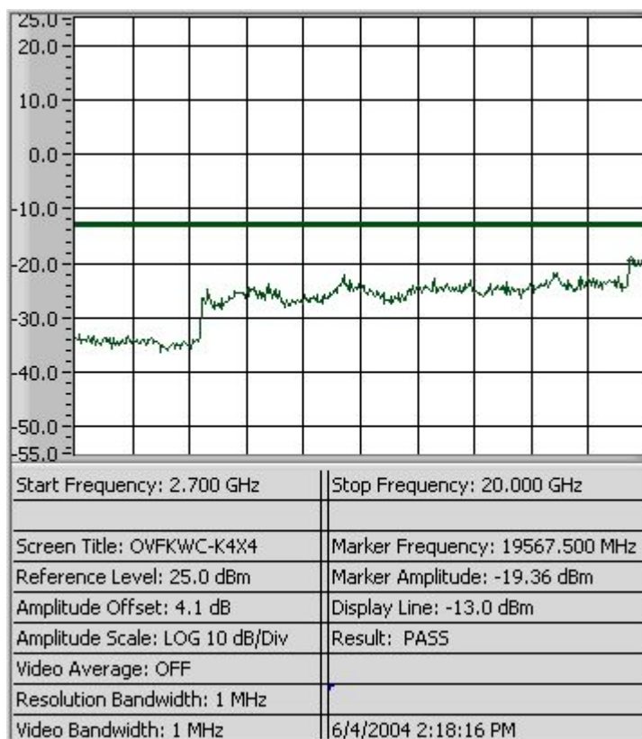
Figure 9-13b CDMA 1900 - Conducted Spurious Emission (CH 25)
