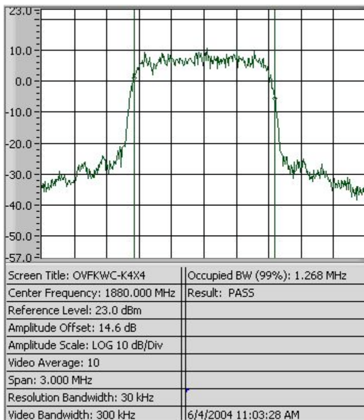
Figure 8-11 CDMA 1900 1X at RC3
