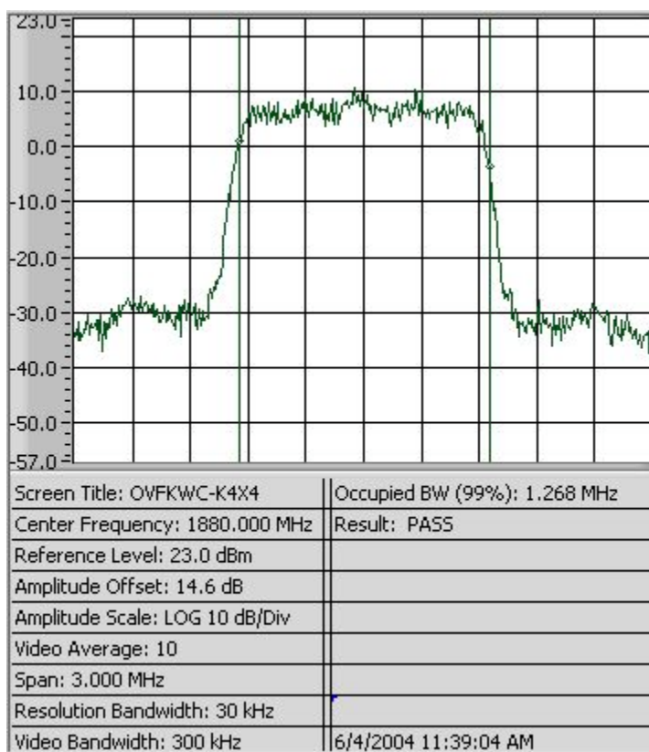
Figure 8-10 CDMA 1900 at RC1
