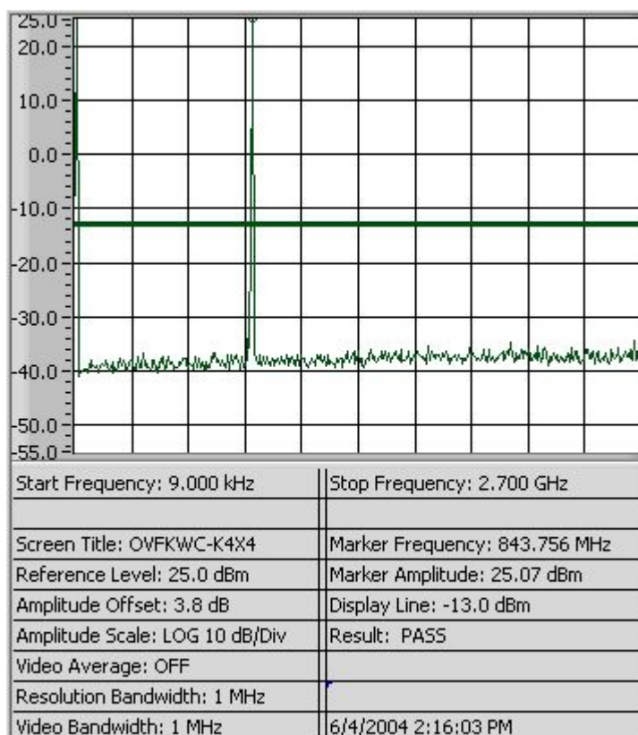
Figure 9-10a CDMA 800 – Conducted Spurious Emission (CH 383)
