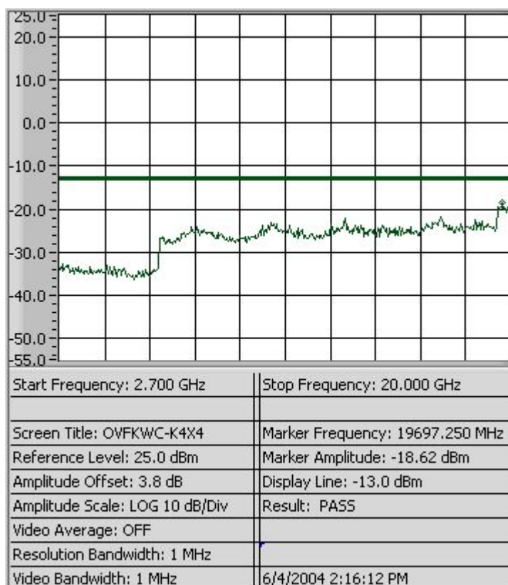
Figure 9-10b CDMA 800 – Conducted Spurious Emission (CH 383)
