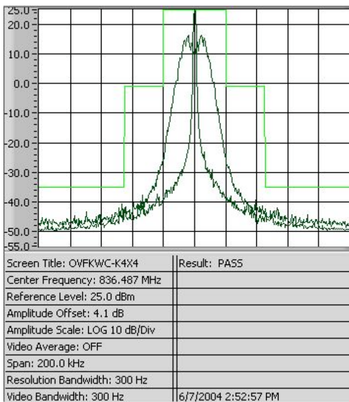
Figure 8-3 AMPS Voice + SAT
