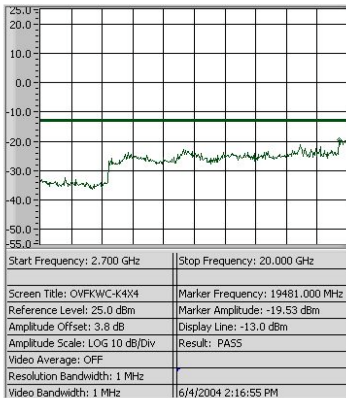
Figure 9-12b CDMA 800 – Conducted Spurious Emission (CH 777)
