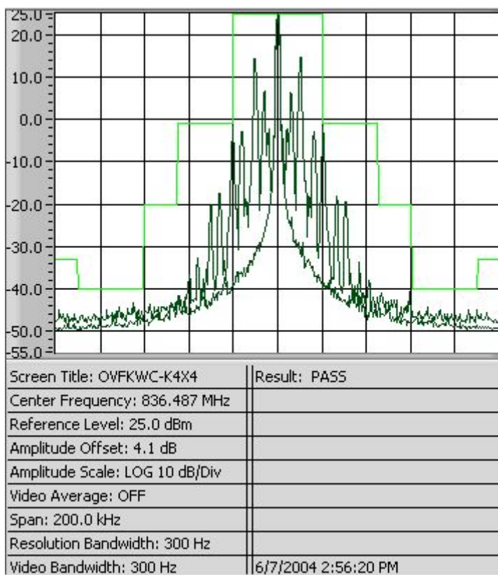
Figure 8-5 AMPS ST + SAT
