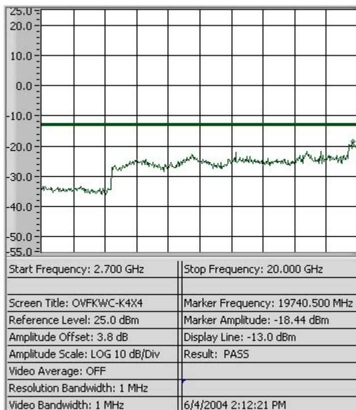
Figure 9-4b AMPS – Conducted Spurious Emission (CH 383)
