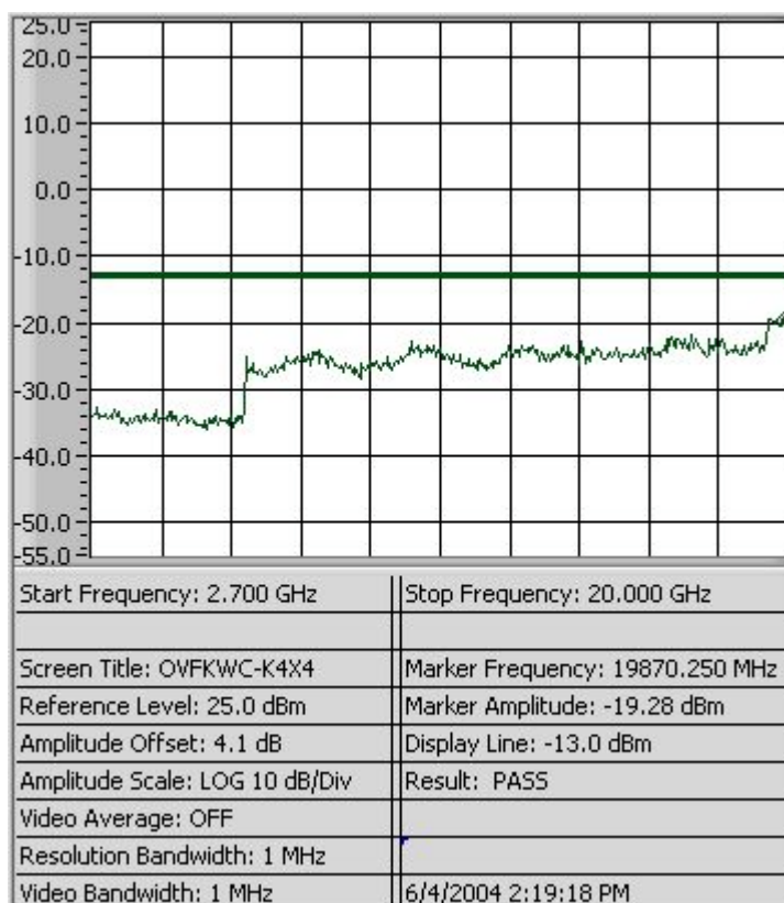
Figure 9-14b CDMA 1900 - Conducted Spurious Emission (CH 600)
