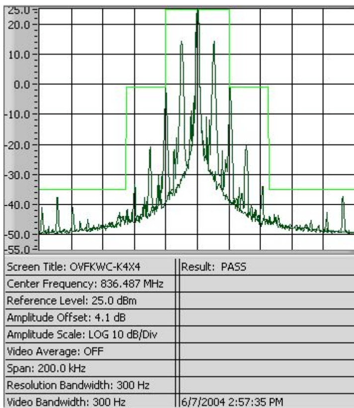
Figure 8-4 AMPS ST
