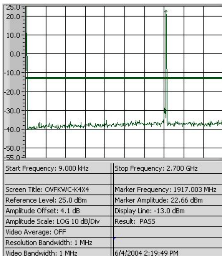
Figure 9-15a CDMA 1900 - Conducted Spurious Emission (CH 1175)
