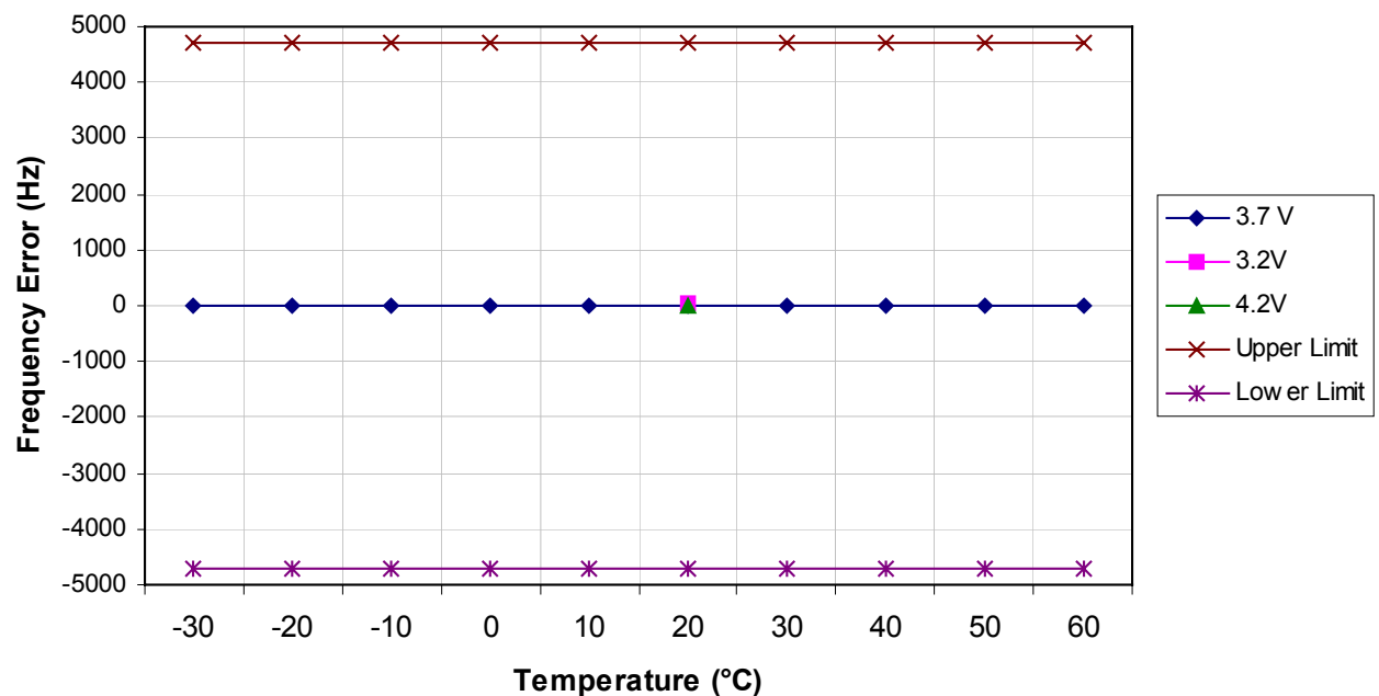
OVFKWC-K4X4 CDMA 1900 MHz Transmit RF Carrier Stability Over Temperature and Voltage
