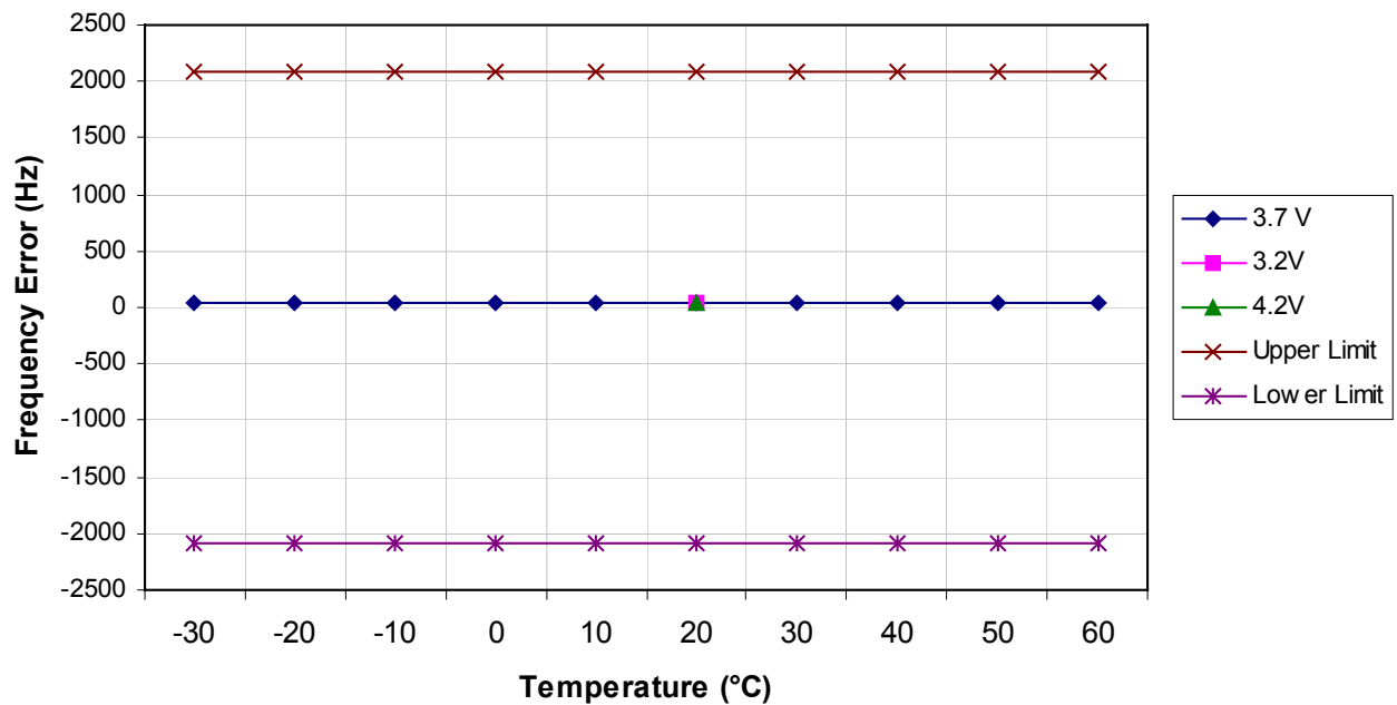
OVFKWC-K4X4 AMPS 800 MHz Transmit RF Carrier Stability Over Temperature and Voltage
