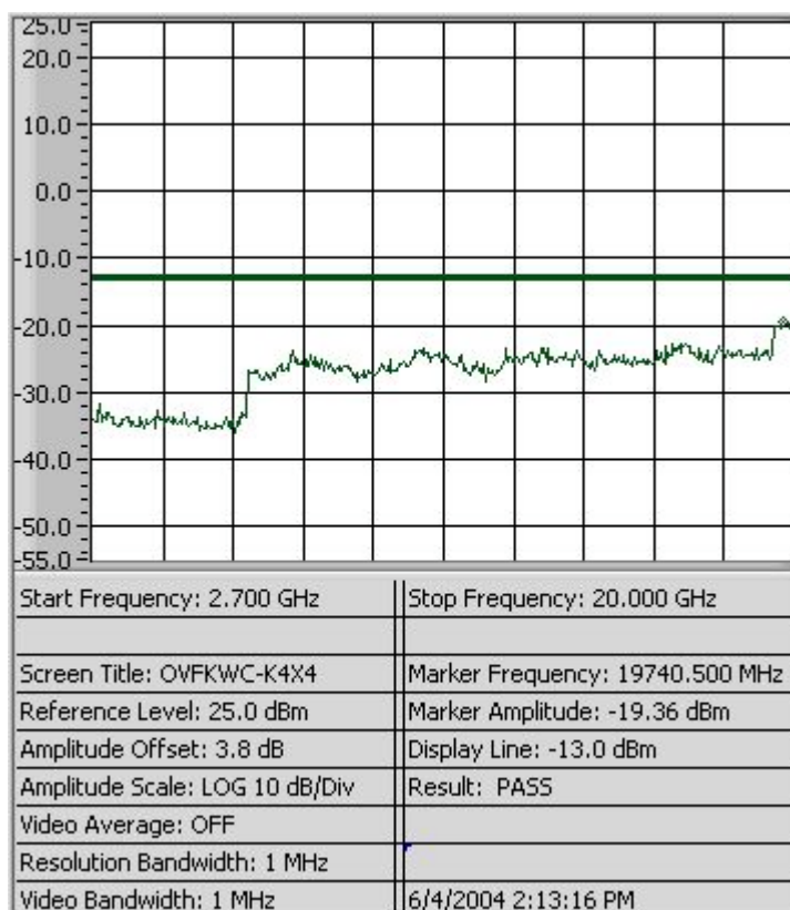
Figure 9-2b AMPS – Conducted Spurious Emission (CH 991)
