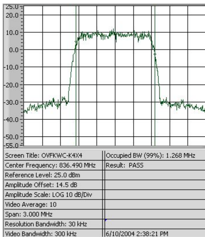
Figure 8-8 CDMA 800 at RC1
