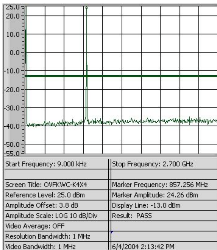
Figure 9-6a AMPS – Conducted Spurious Emission (CH 799)
