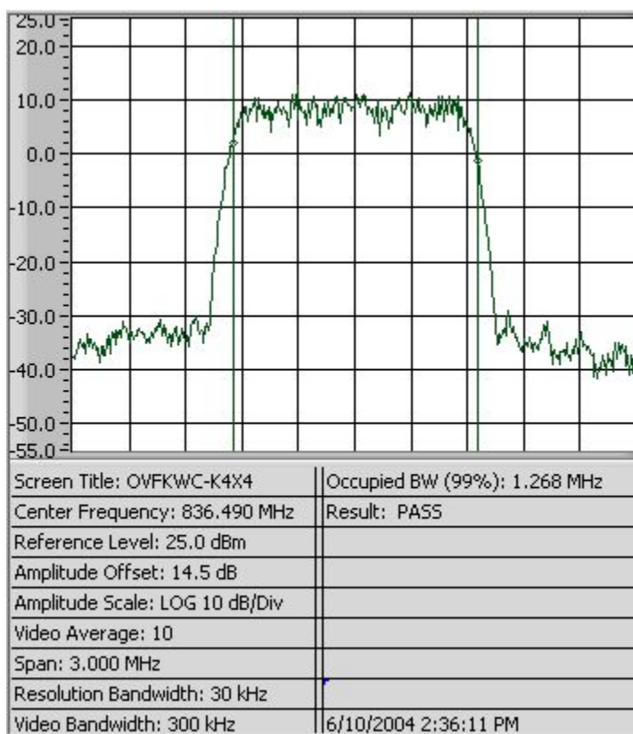
Figure 8-9 CDMA 800 1X at RC3
