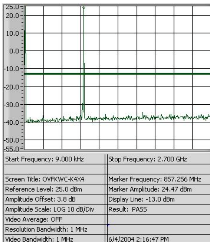
Figure 9-12a CDMA 800 – Conducted Spurious Emission (CH 777)
