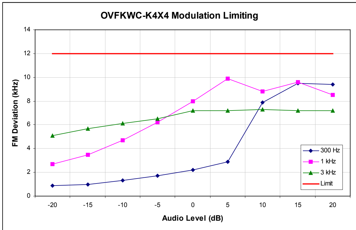
Figure 7.3 Modulation Deviation Limiting
