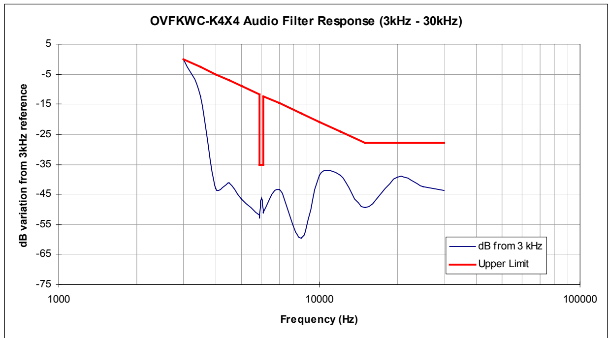
Figure 7.2 Post Limiter Filter Attenuation
