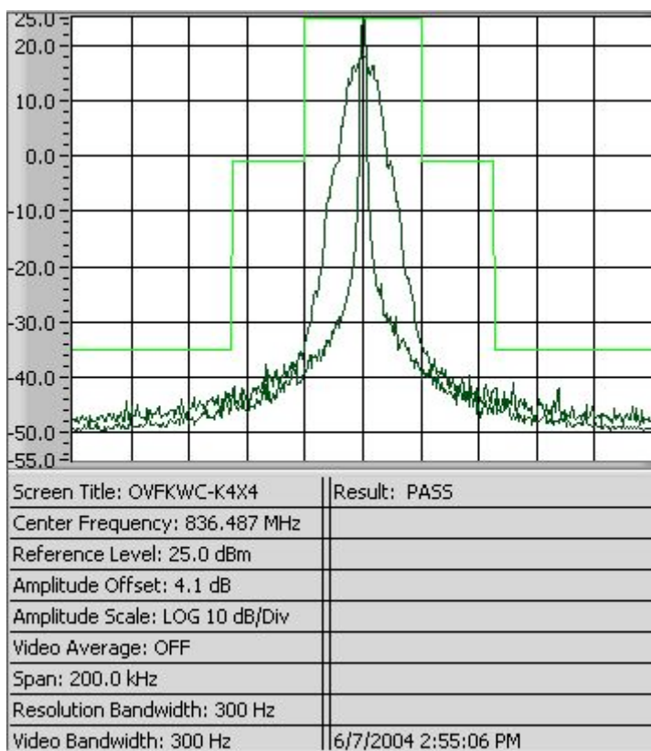
Figure 8-6 SAT + DTMF_9
