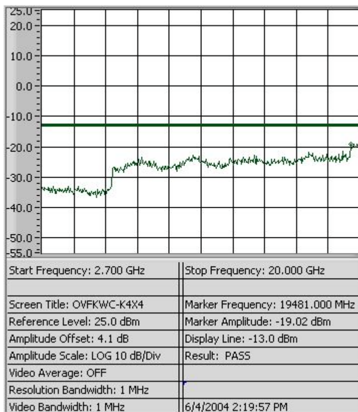
Figure 9-15b CDMA 1900 - Conducted Spurious Emission (CH 1175)
