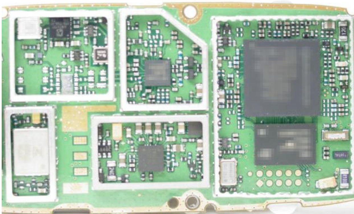
PCB side 1 with shields off
