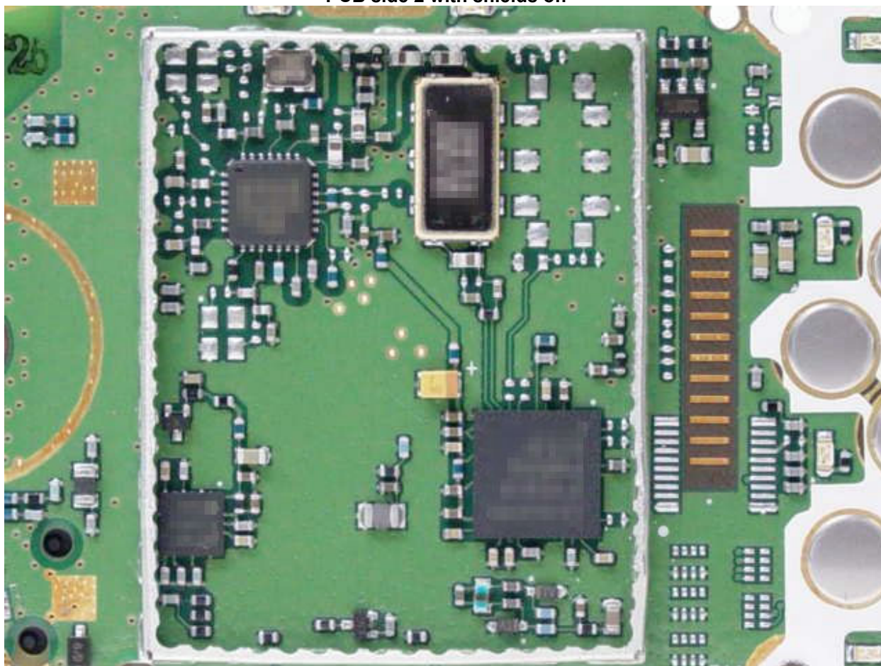
PCB side 2 with shields off
