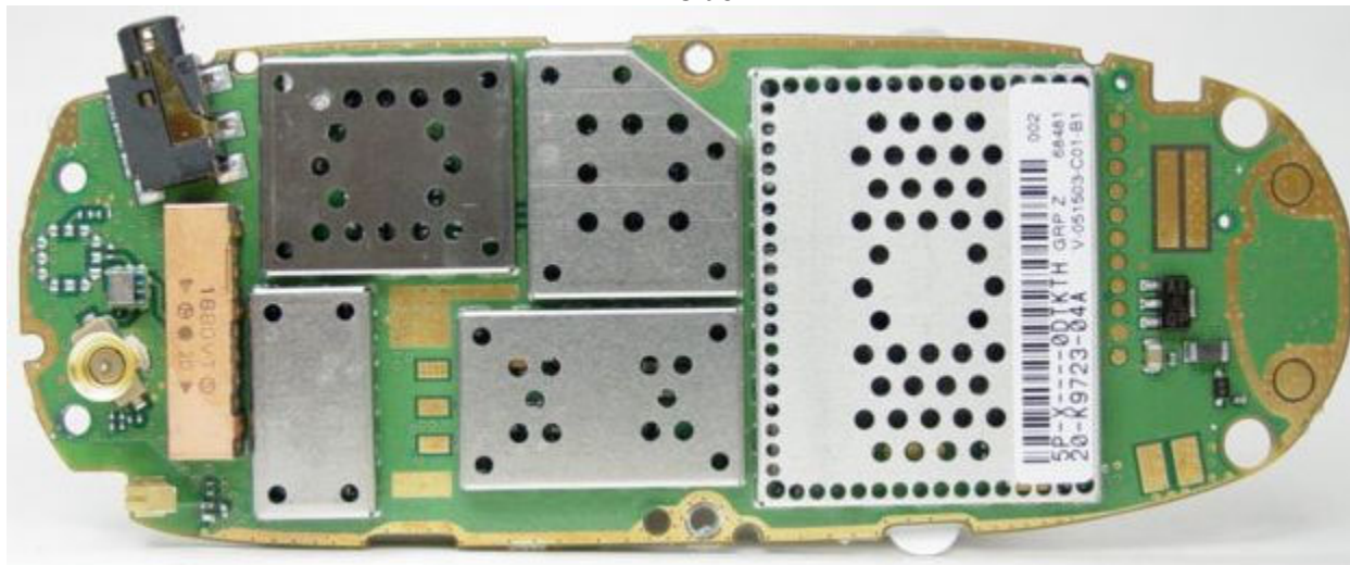
PCB side 1
