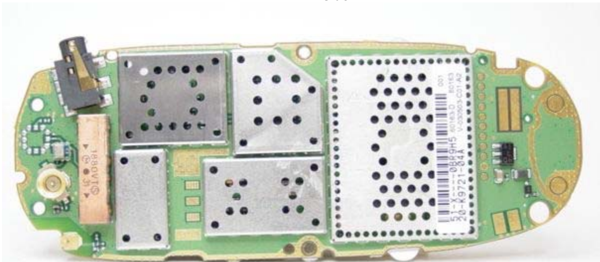
KE414 PCB side 1
