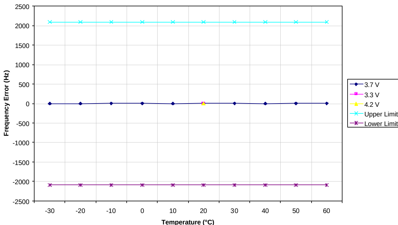
OVFKWC-KX16 CDMA 800 MHz Transmit RF Carrier Stability Over Temperature and Voltage
