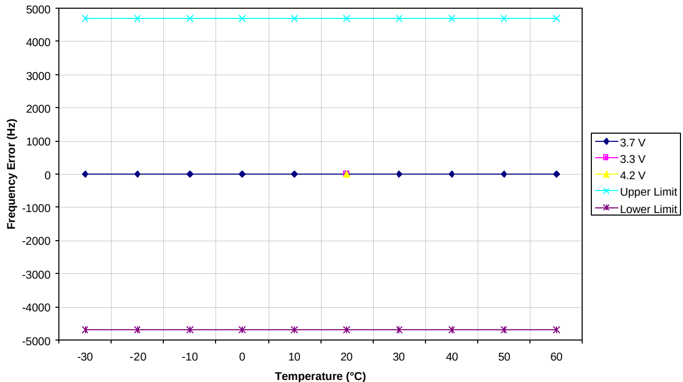
OVFKWC-KX16 CDMA 1900 MHz Transmit RF Carrier Stability Over Temperature and Voltage
