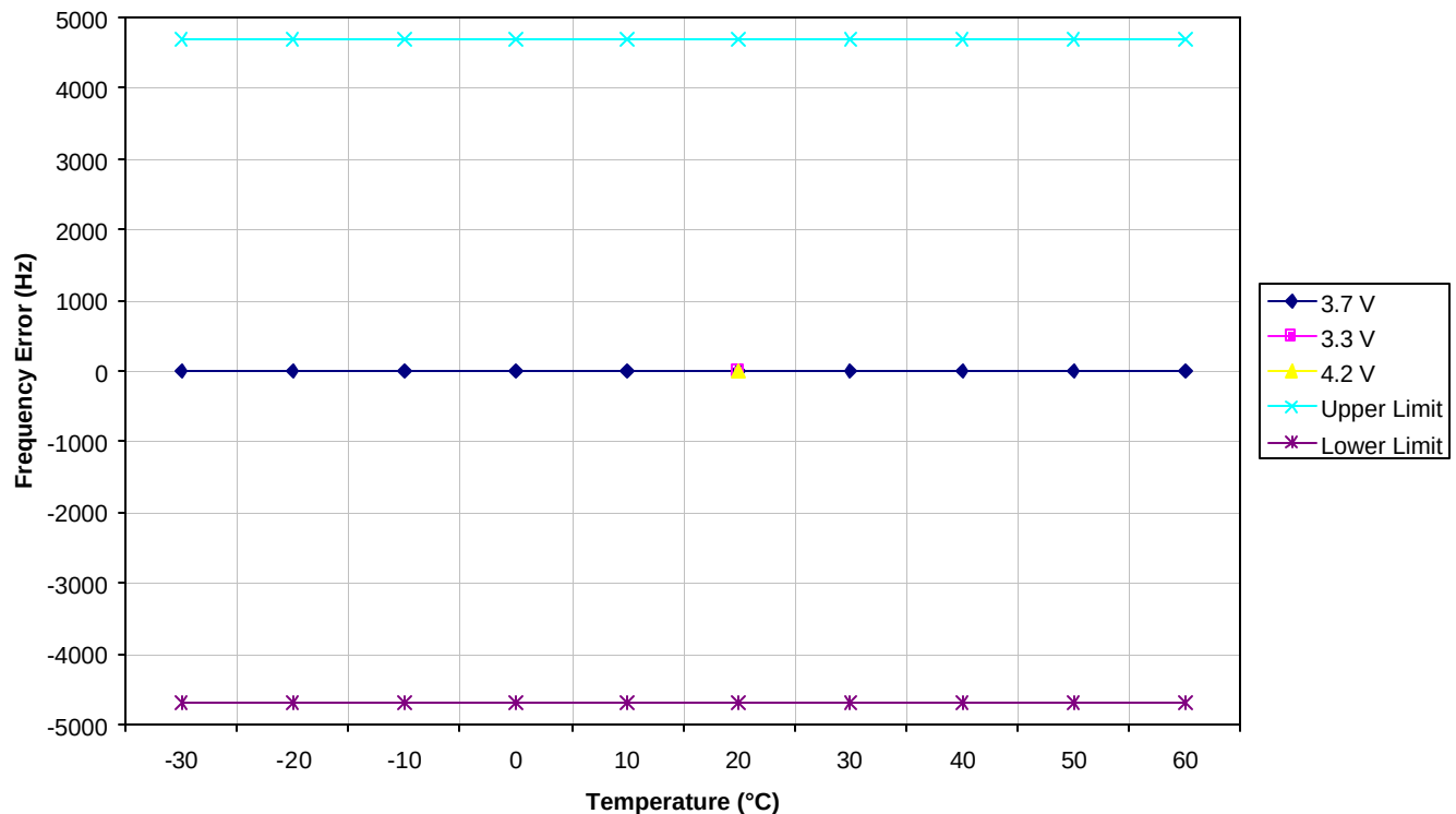
OVFKWC-KX160A CDMA 1900 MHz Transmit RF Carrier Stability Over Temperature and Voltage
