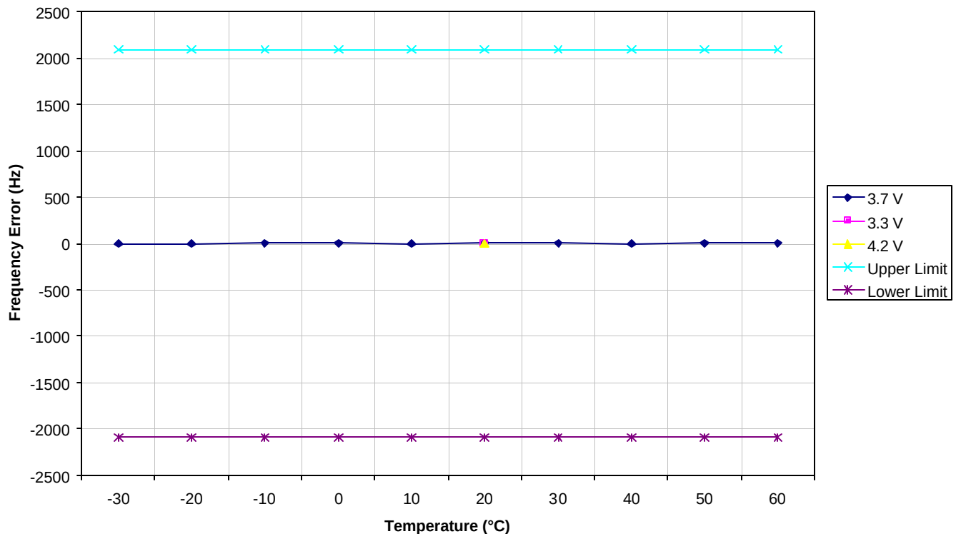
OVFKWC-KX160A CDMA 800 MHz Transmit RF Carrier Stability Over Temperature and Voltage
