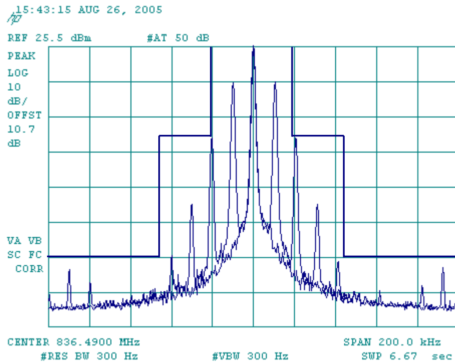
Figure 7-4 AMPS ST
