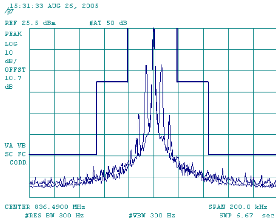
Figure 7-2 AMPS SAT
