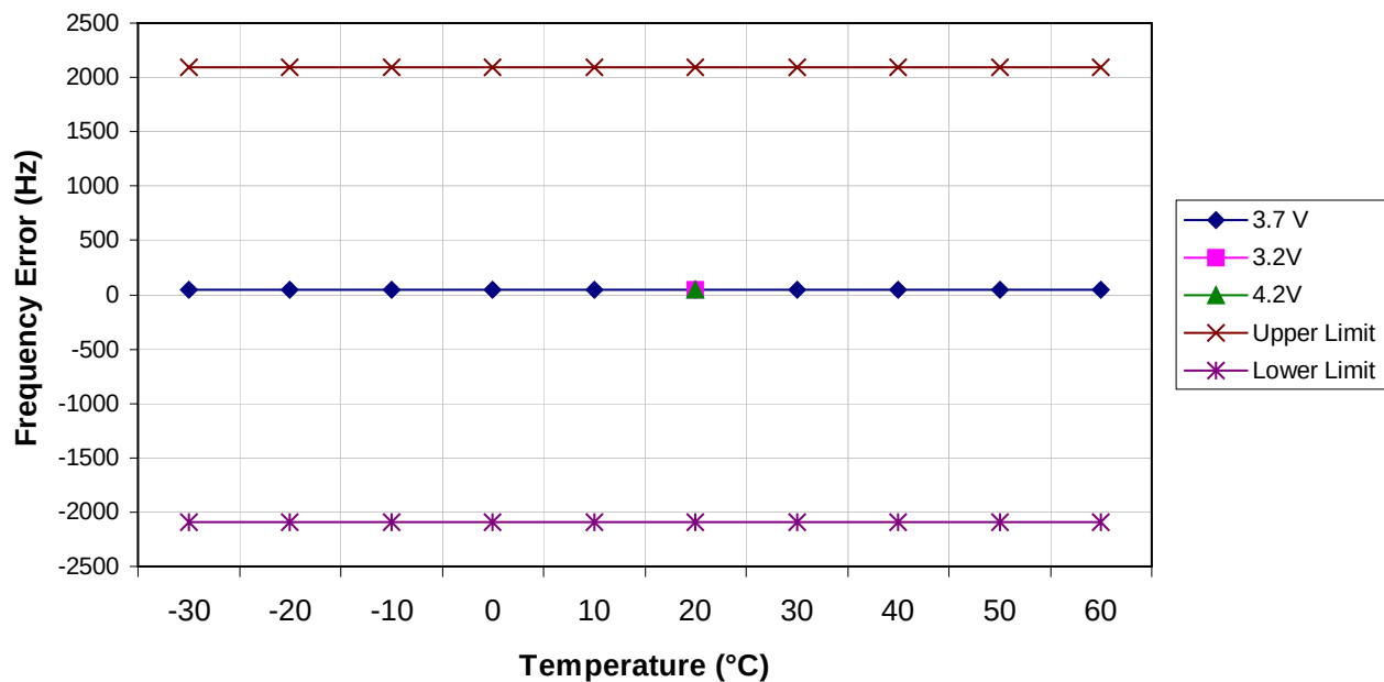
OVFKWC-KX160B AMPS 800 MHz Transmit RF Carrier Stability Over Temperature and Voltage
