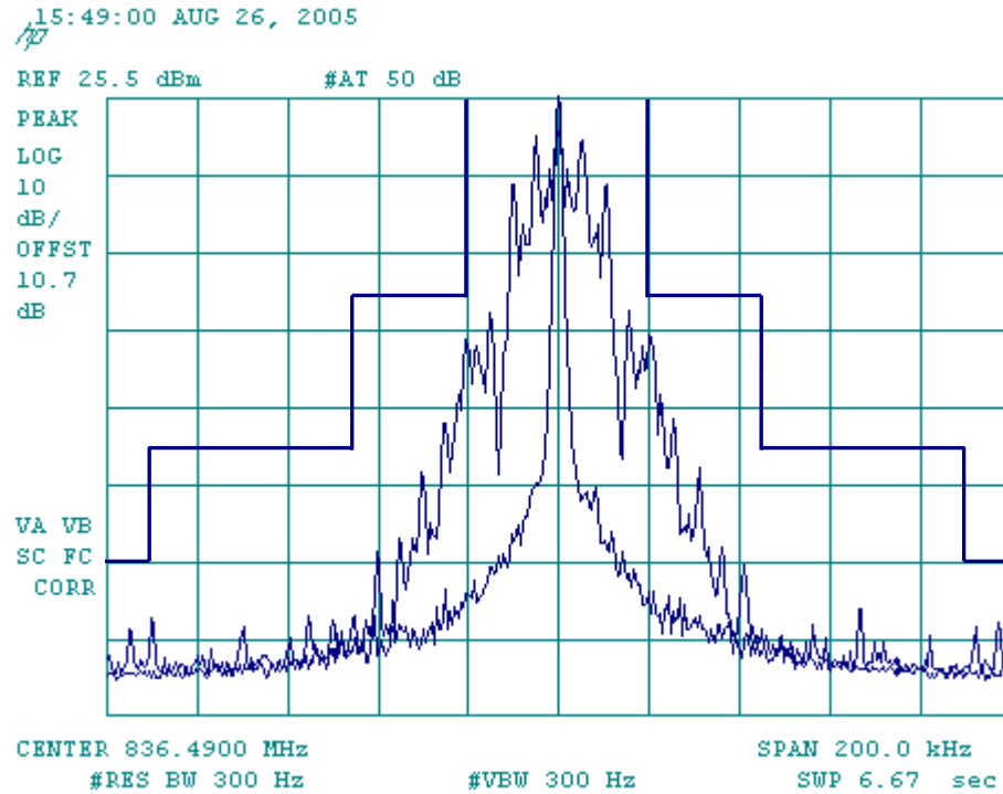
Figure 7-7 AMPS WIDEBAND
