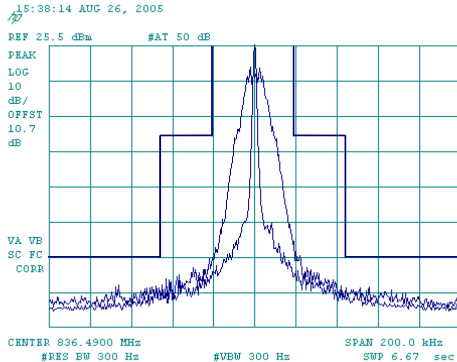
Figure 7-6 SAT + DTMF_9
