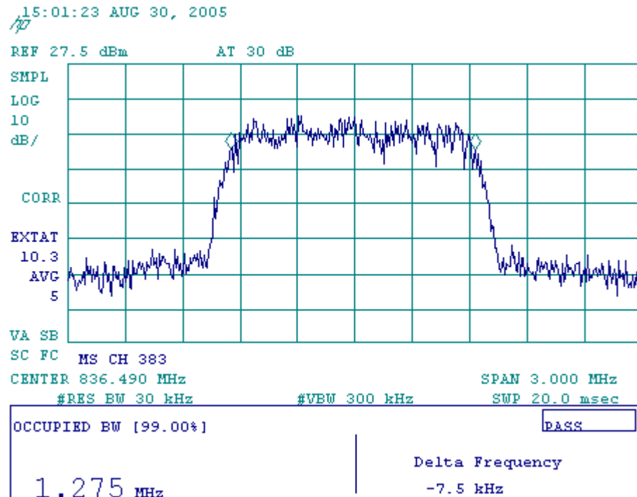
Figure 7-8 CDMA 800 @ CH 383
