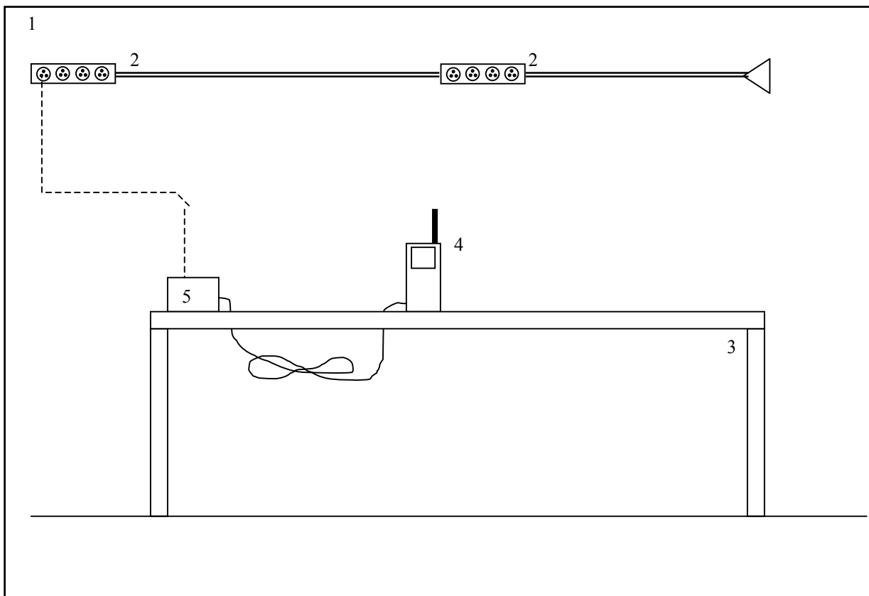
Figure 1. General EUT Test Setup Diagram
